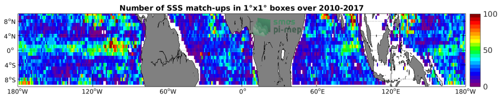
Figure 4: Number of SSS match-ups between Argo SSS and the SMOS L4 v2 Weekly (CATDS-CECOS-IFREMER) SSS product for the Equatorial Ocean 10N-10S Pi-MEP region over 1°x1° boxes and for the full satellite product period.
