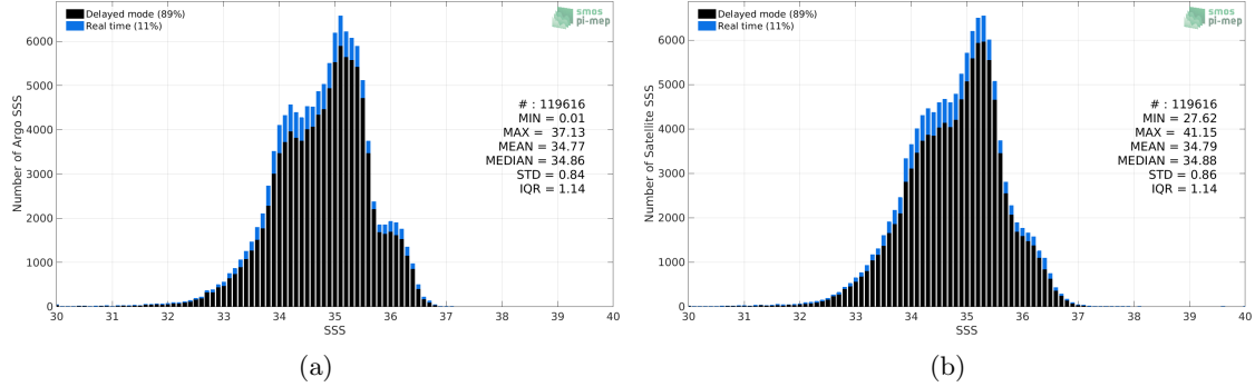
Figure 2: Histograms of SSS from Argo (a) and SMOS L4 v2 Weekly (CATDS-CECOS-IFREMER) (b) considering all match-up pairs per bins of 0.1 over the Equatorial Ocean 10N-10S Pi-MEP region and for the full satellite product period.
