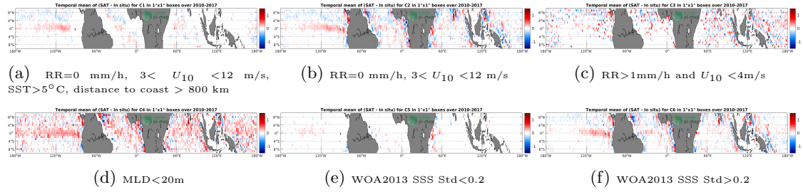
Figure 12: Temporal mean gridded over spatial boxes of size 1^\circ \times 1^\circ of \Delta SSS (SMOS L4 v2 Weekly (CATDS-CECOS-IFREMER) - Argo) for 6 different subdatasets corresponding to: RR=0 mm/h, 3 < U_{10} < 12 m/s, SST >5^\circ\text{C} , distance to coast > 800 km (a), RR=0 mm/h, 3 < U_{10} < 12 m/s (b), RR >1 mm/h and U_{10} < 4 m/s (c),MLD <20 m (d),WOA2013 SSS Std <0.2 (e),WOA2013 SSS Std >0.2 (f).
