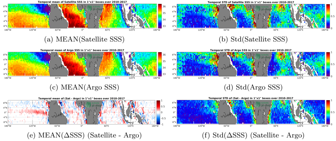
Figure 6: Temporal mean (left) and Std (right) of SSS from SMOS L4 v2 Weekly (CATDS-CECOS-IFREMER) (top), Argo (middle), and of \Delta SSS (Satellite - Argo). Only match-up pairs are used to generate these maps.
