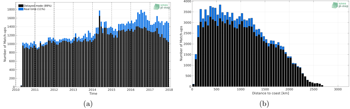
Figure 1: Number of match-ups between Argo and SMOS L4 v2 Weekly (CATDS-CECOS-IFREMER) SSS as a function of time (a) and as function of the distance to coast (b) over the Equatorial Ocean 10N-10S Pi-MEP region and for the full satellite product period.
