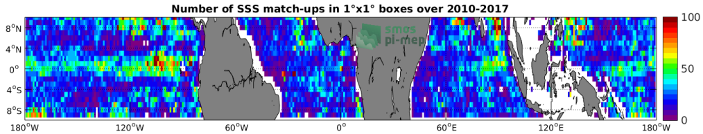
Figure 4: Number of SSS match-ups between Argo SSS and the SMOS-L4-CATDS-CECOS-IFREMER-V2-WEEKLY-0.5DEG SSS product for the Equatorial Ocean 10N-10S Pi-MEP region over 1°x1° boxes and for the full satellite product period.
