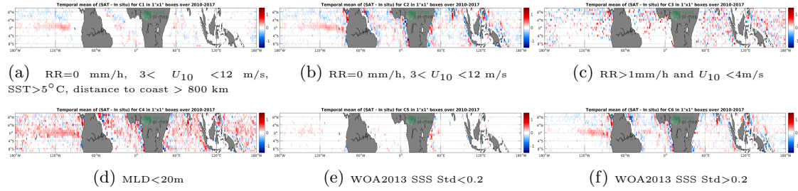
Figure 12: Temporal mean gridded over spatial boxes of size 1^\circ \times 1^\circ of \Delta SSS (SMOS-L4-CATDS-CECOS-IFREMER-V2-WEEKLY-0.5DEG - Argo) for 6 different subdatasets corresponding to: RR=0 mm/h, 3 < U_{10} < 12 m/s, SST > 5^\circ C , distance to coast > 800 km (a), RR=0 mm/h, 3 < U_{10} < 12 m/s (b), RR > 1 mm/h and U_{10} < 4 m/s (c), MLD < 20 m (d), WOA2013 SSS Std < 0.2 (e), WOA2013 SSS Std > 0.2 (f).
