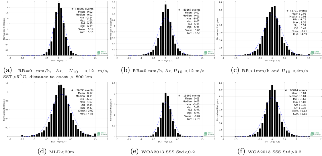
Figure 13: Normalized histogram of \Delta SSS (SMOS-L4-CATDS-CECOS-IFREMER-V2-WEEKLY-0.5DEG - Argo) for 6 different subdatasets corresponding to: RR=0 mm/h, 3 < U_{10} < 12 m/s, SST > 5^\circ C , distance to coast > 800 km (a), RR=0 mm/h, 3 < U_{10} < 12 m/s (b), RR > 1 mm/h and U_{10} < 4 m/s (c), MLD < 20 m (d), WOA2013 SSS Std <0.2 (e), WOA2013 SSS Std >0.2 (f).
