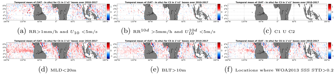
Figure 12: Temporal mean gridded over spatial boxes of size 1^\circ \times 1^\circ of \Delta SSS (SMOS-L4-CATDS-CECOS-IFREMER-V2-WEEKLY-0.5DEG - Argo) for 6 different subdatasets corresponding to: RR > 1\text{mm/h} and U_{10} < 5\text{m/s} (a), RR^{10d} > 5\text{mm/h} and U_{10}^{10d} < 5\text{m/s} (b), C1 U C2 (c), MLD < 20\text{m} (d), BLT > 10\text{m} (e), Locations where WOA2013 SSS STD > 0.2 (f).
