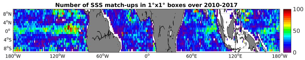
Figure 4: Number of SSS match-ups between Argo SSS and the SMOS-L4-CATDS-CECOS-IFREMER-V2-WEEKLY-0.5DEG SSS product for the Equatorial Ocean 10N-10S Pi-MEP region over 1°x1° boxes and for the full satellite product period.
