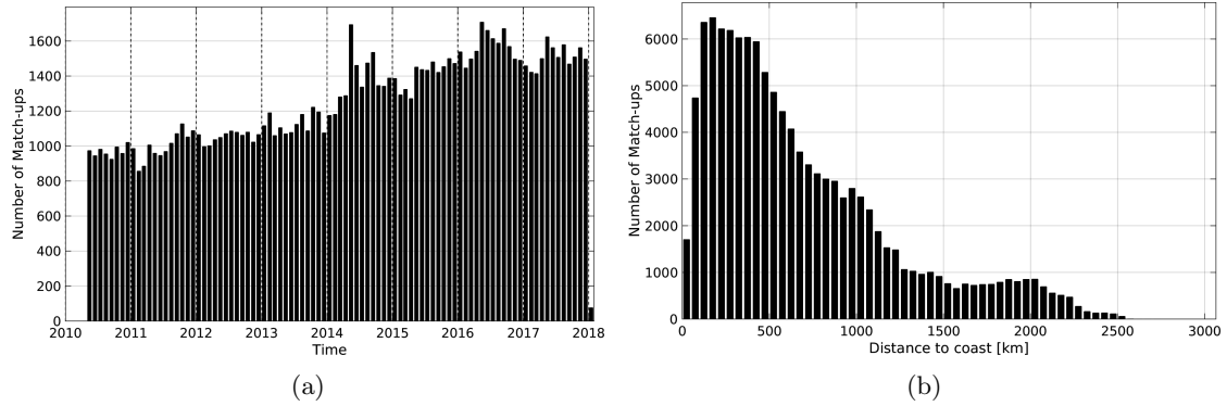
Figure 1: Number of match-ups between Argo and SMOS-L4-CATDS-CECOS-IFREMER-V2-WEEKLY-0.5DEG SSS as a function of time (a) and as function of the distance to coast (b) over the Equatorial Ocean 10N-10S Pi-MEP region and for the full satellite product period.
