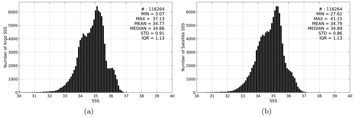
Figure 2: Histograms of SSS from Argo (a) and SMOS-L4-CATDS-CECOS-IFREMER-V2-WEEKLY-0.5DEG (b) considering all match-up pairs per bins of 0.1 over the Equatorial Ocean 10N-10S Pi-MEP region and for the full satellite product period.
