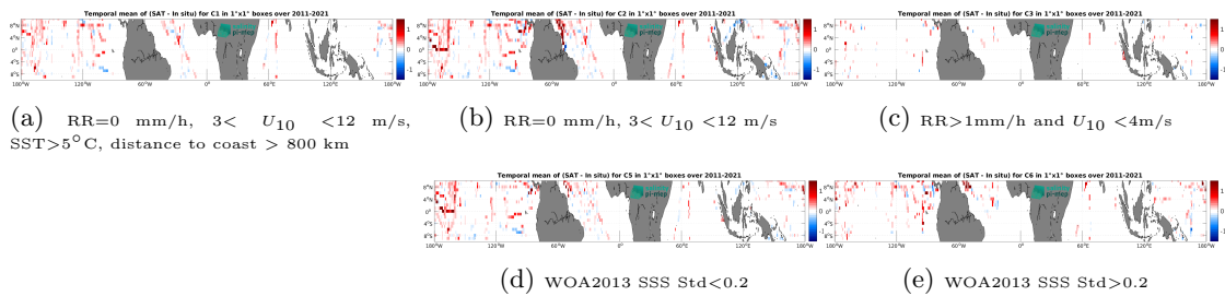
Figure 14: Temporal mean gridded over spatial boxes of size 1^\circ \times 1^\circ of \Delta\text{SSS} (SMOS SSS L4 v2 - Daily (BEC) - TSG (SAMOS)) for 5 different subdatasets corresponding to:RR=0 mm/h, 3 < U_{10} < 12 m/s, SST>5°C, distance to coast > 800 km (a), RR=0 mm/h, 3 < U_{10} < 12 m/s (b), RR>1mm/h and U_{10} < 4 m/s (c), WOA2013 SSS Std<0.2 (d), WOA2013 SSS Std>0.2 (e).
