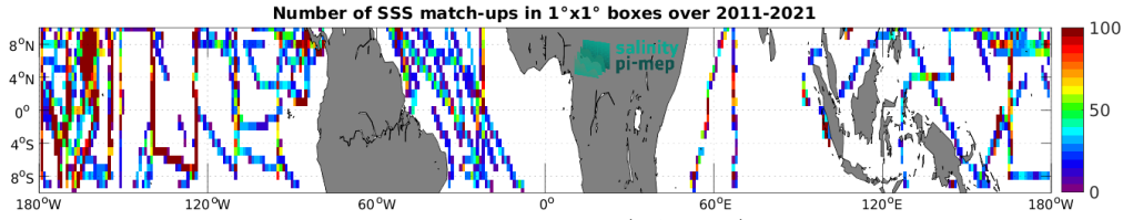
Figure 5: Number of SSS match-ups between TSG (SAMOS) SSS and the SMOS SSS L4 v2 - Daily (BEC) SSS product for the Equatorial Ocean 10N-10S Pi-MEP region over 1^\circ \times 1^\circ boxes and for the full satellite product period.
