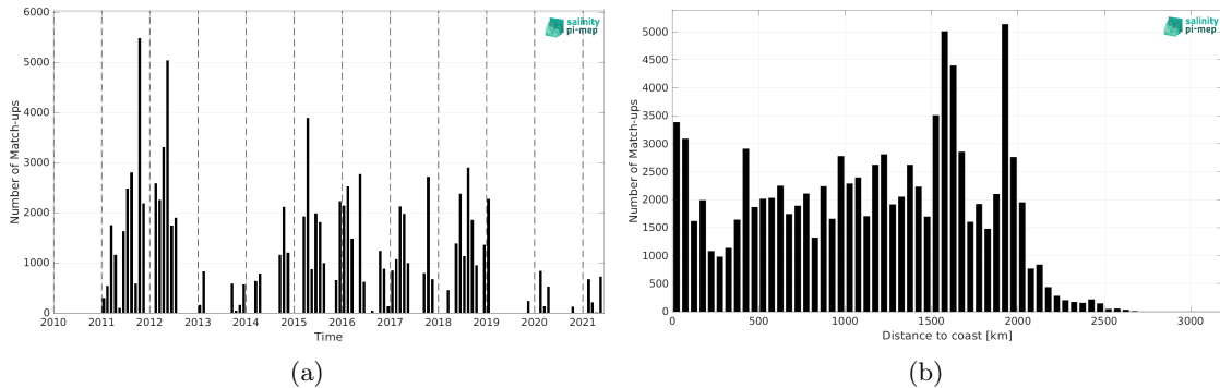
Figure 2: Number of match-ups between TSG (SAMOS) and SMOS SSS L4 v2 - Daily (BEC) SSS as a function of time (a) and as function of the distance to coast (b) over the Equatorial Ocean 10N-10S Pi-MEP region and for the full satellite product period.
