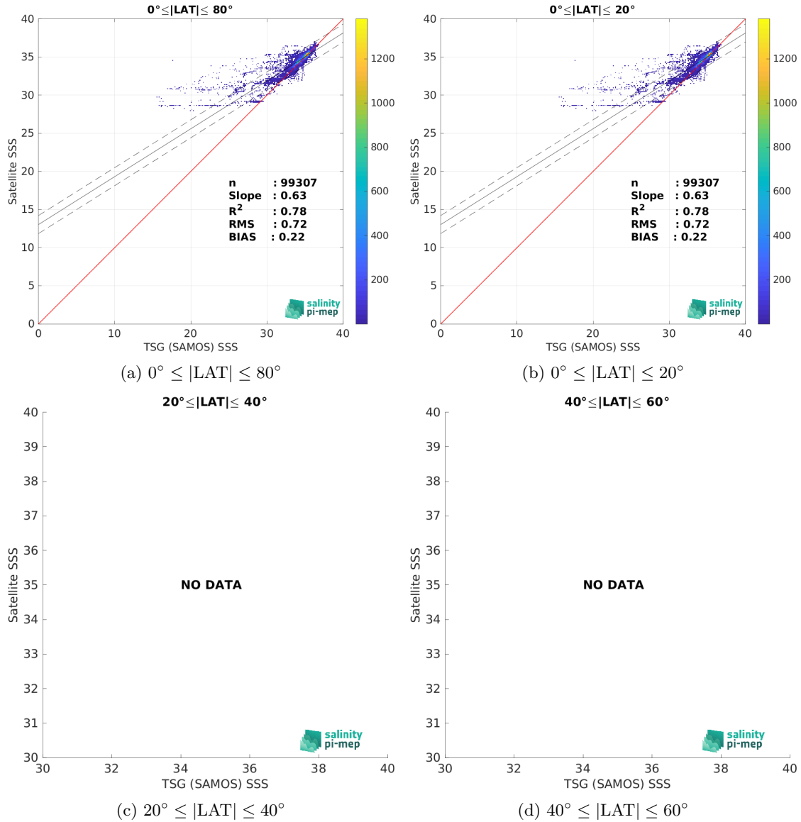
Figure 10: Contour maps of the concentration of SMOS SSS L4 v2 - Daily (BEC) SSS (y-axis) versus TSG (SAMOS) SSS (x-axis) at match-up pairs for different latitude bands. For each plot, the red line shows x=y . The black thin and dashed lines indicate a linear fit through the data cloud and the \pm 95\% confidence levels, respectively. The number match-up pairs n , the slope and R^2 coefficient of the linear fit, the root mean square (RMS) and the mean bias between satellite and in situ data are indicated for each latitude band in each plots.
