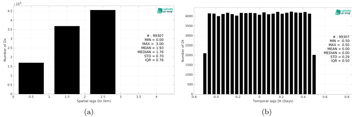
Figure 6: Histograms of the spatial (a) and temporal (b) lags between the location/time of the TSG (SAMOS) measurement and the date of the corresponding SMOS SSS L4 v2 - Daily (BEC) SSS pixel.
