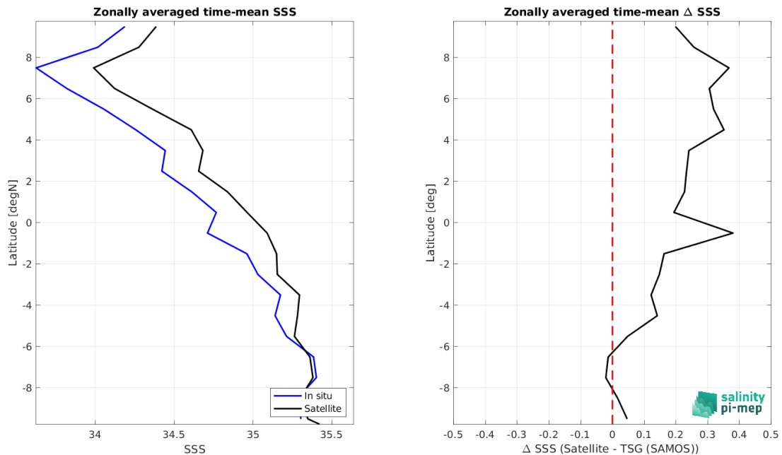
Figure 9: Left panel: Zonal mean SSS from SMOS SSS L4 v2 - Daily (BEC) satellite product (black) and from TSG (SAMOS) (blue). Right panel: Zonal mean of \Delta SSS (Satellite - TSG (SAMOS)) for all the collected Pi-MEP match-up pairs estimated over the full satellite product period.
