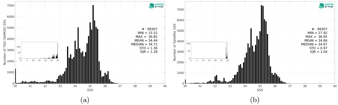
Figure 3: Histograms of SSS from TSG (SAMOS) (a) and SMOS SSS L4 v2 - Daily (BEC) (b) considering all match-up pairs per bins of 0.1 over the Equatorial Ocean 10N-10S Pi-MEP region and for the full satellite product period.
