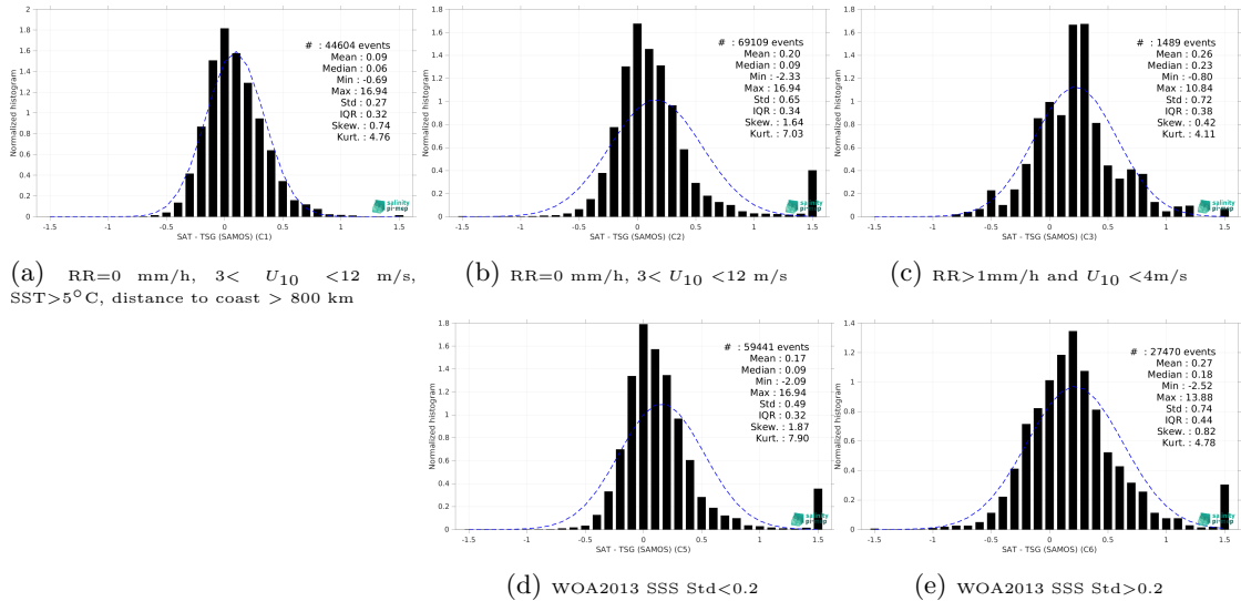
Figure 15: Normalized histogram of \Delta\text{SSS} (SMOS SSS L4 v2 - Daily (BEC) - TSG (SAMOS)) for 5 different subdatasets corresponding to: RR=0 mm/h, 3 < U_{10} < 12 m/s, SST>5°C, distance to coast > 800 km (a), RR=0 mm/h, 3 < U_{10} < 12 m/s (b), RR>1mm/h and U_{10} < 4 m/s (c), WOA2013 SSS Std<0.2 (d), WOA2013 SSS Std>0.2 (e).
