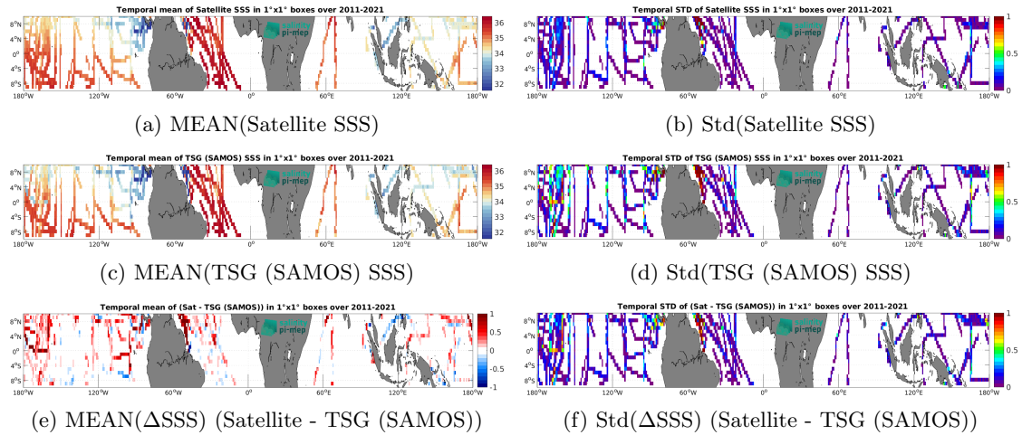
Figure 7: Temporal mean (left) and Std (right) of SSS from SMOS SSS L4 v2 - Daily (BEC) (top), TSG (SAMOS) (middle), and of \Delta SSS (Satellite - TSG (SAMOS)). Only match-up pairs are used to generate these maps.
