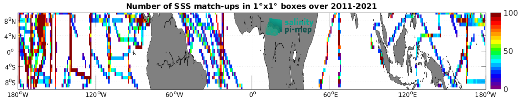
Figure 4: Number of SSS match-ups between TSG (SAMOS) SSS and the SMOS SSS L4 v2 - Daily (BEC) SSS product for the Equatorial Ocean 10N-10S Pi-MEP region over 1^\circ \times 1^\circ boxes and for the full satellite product period.
