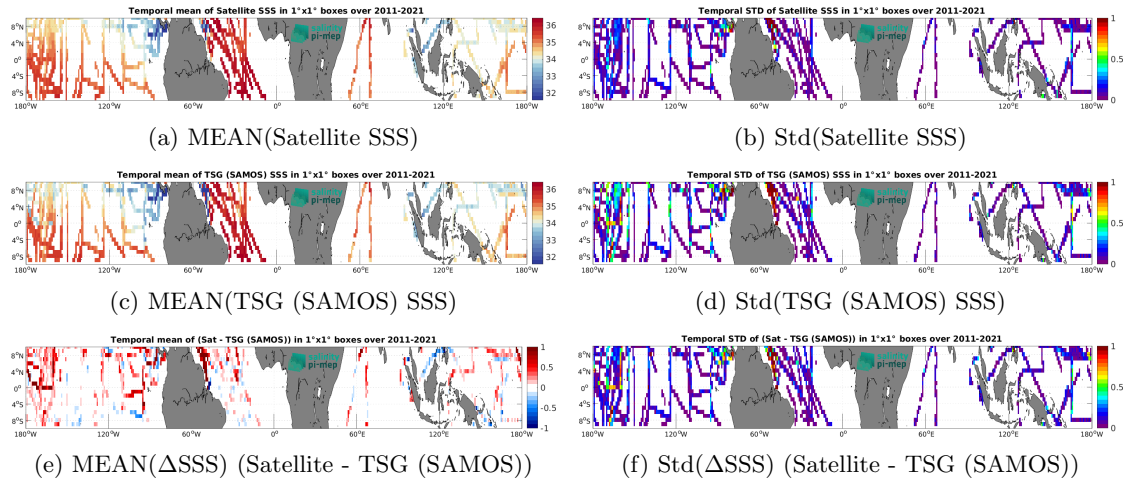
Figure 6: Temporal mean (left) and Std (right) of SSS from SMOS SSS L4 v2 - Daily (BEC) (top), TSG (SAMOS) (middle), and of \Delta SSS (Satellite - TSG (SAMOS)). Only match-up pairs are used to generate these maps.
