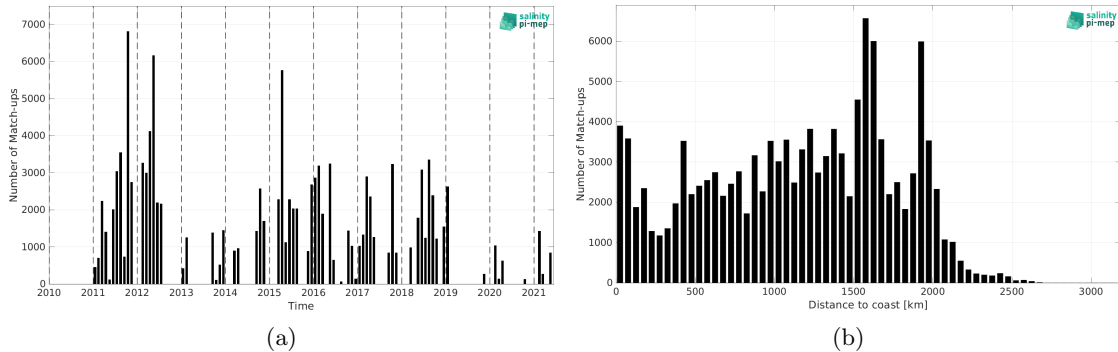
Figure 1: Number of match-ups between TSG (SAMOS) and SMOS SSS L4 v2 - Daily (BEC) SSS as a function of time (a) and as function of the distance to coast (b) over the Equatorial Ocean 10N-10S Pi-MEP region and for the full satellite product period.
