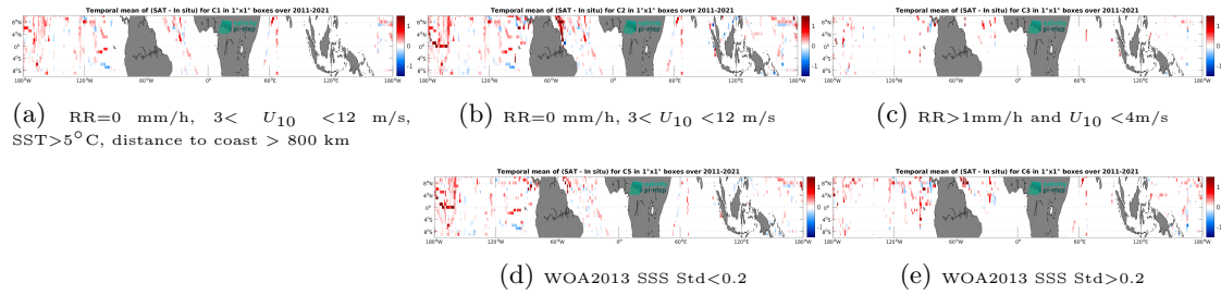
Figure 12: Temporal mean gridded over spatial boxes of size 1^\circ \times 1^\circ of \Delta\text{SSS} (SMOS SSS L4 v2 - Daily (BEC) - TSG (SAMOS)) for 5 different subdatasets corresponding to:RR=0 mm/h, 3 < U_{10} < 12 m/s, \text{SST} > 5^\circ\text{C} , distance to coast > 800 km (a), RR=0 mm/h, 3 < U_{10} < 12 m/s (b), RR>1mm/h and U_{10} < 4 m/s (c), WOA2013 SSS Std<0.2 (d), WOA2013 SSS Std>0.2 (e).
