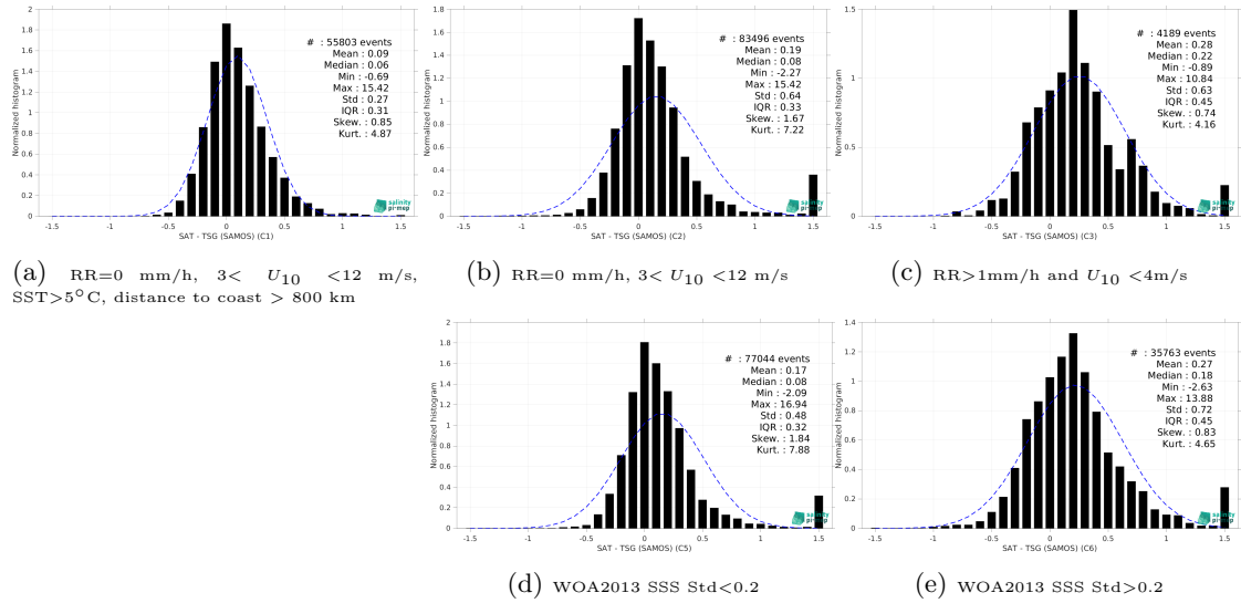
Figure 13: Normalized histogram of \Delta\text{SSS} (SMOS SSS L4 v2 - Daily (BEC) - TSG (SAMOS)) for 5 different subdatasets corresponding to: RR=0 mm/h, 3 < U_{10} < 12 m/s, \text{SST} > 5^\circ\text{C} , distance to coast > 800 km (a), RR=0 mm/h, 3 < U_{10} < 12 m/s (b), RR>1mm/h and U_{10} < 4 m/s (c), WOA2013 SSS Std<0.2 (d), WOA2013 SSS Std>0.2 (e).
