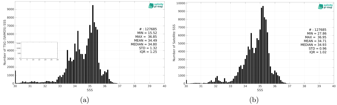
Figure 2: Histograms of SSS from TSG (SAMOS) (a) and SMOS SSS L4 v2 - Daily (BEC) (b) considering all match-up pairs per bins of 0.1 over the Equatorial Ocean 10N-10S Pi-MEP region and for the full satellite product period.
