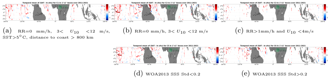
Figure 12: Temporal mean gridded over spatial boxes of size 1^\circ \times 1^\circ of \Delta SSS (SMOS SSS L4 v2 - Daily (BEC) - TSG (SAMOS)) for 5 different subdatasets corresponding to: RR=0 mm/h, 3 < U_{10} < 12 m/s, SST > 5^\circ C , distance to coast > 800 km (a), RR=0 mm/h, 3 < U_{10} < 12 m/s (b), RR > 1 mm/h and U_{10} < 4 m/s (c), WOA2013 SSS Std < 0.2 (d), WOA2013 SSS Std > 0.2 (e).
