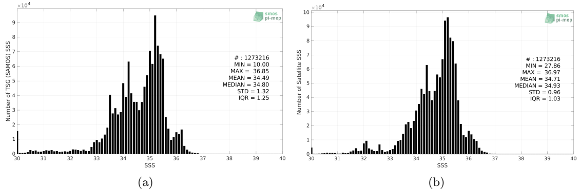
Figure 2: Histograms of SSS from TSG (SAMOS) (a) and SMOS SSS L4 v2 - Daily (BEC) (b) considering all match-up pairs per bins of 0.1 over the Equatorial Ocean 10N-10S Pi-MEP region and for the full satellite product period.
