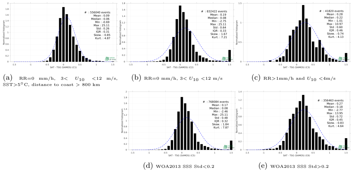
Figure 13: Normalized histogram of \Delta SSS (SMOS SSS L4 v2 - Daily (BEC) - TSG (SAMOS)) for 5 different subdatasets corresponding to: RR=0 mm/h, 3 < U_{10} < 12 m/s, SST > 5^\circ C , distance to coast > 800 km (a), RR=0 mm/h, 3 < U_{10} < 12 m/s (b), RR > 1 mm/h and U_{10} < 4 m/s (c), WOA2013 SSS Std < 0.2 (d), WOA2013 SSS Std > 0.2 (e).
