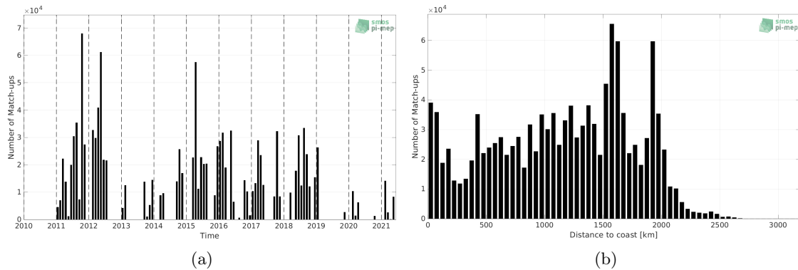
Figure 1: Number of match-ups between TSG (SAMOS) and SMOS SSS L4 v2 - Daily (BEC) SSS as a function of time (a) and as function of the distance to coast (b) over the Equatorial Ocean 10N-10S Pi-MEP region and for the full satellite product period.
