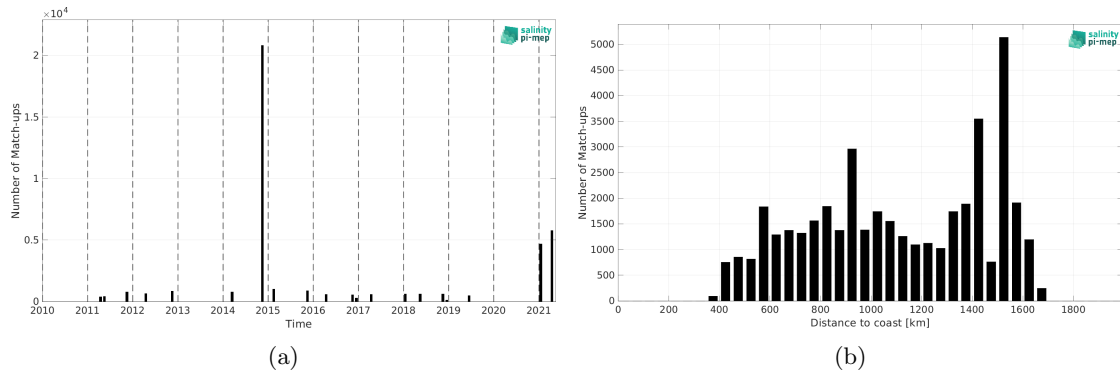
Figure 2: Number of match-ups between TSG (Polarstern) and SMOS SSS L4 v2 - Daily (BEC) SSS as a function of time (a) and as function of the distance to coast (b) over the Equatorial Ocean 10N-10S Pi-MEP region and for the full satellite product period.
