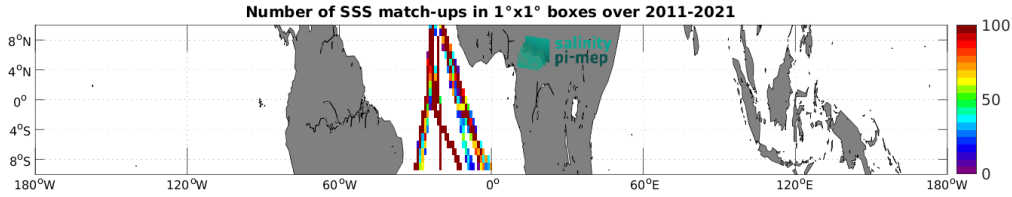
Figure 5: Number of SSS match-ups between TSG (Polarstern) SSS and the SMOS SSS L4 v2 - Daily (BEC) SSS product for the Equatorial Ocean 10N-10S Pi-MEP region over 1^\circ \times 1^\circ boxes and for the full satellite product period.
