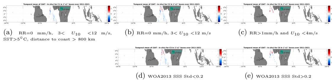
Figure 14: Temporal mean gridded over spatial boxes of size 1^\circ \times 1^\circ of \Delta SSS (SMOS SSS L4 v2 - Daily (BEC) - TSG (Polarstern)) for 5 different subdatasets corresponding to:RR=0 mm/h, 3 < U_{10} < 12 m/s, SST>5°C, distance to coast > 800 km (a), RR=0 mm/h, 3 < U_{10} < 12 m/s (b), RR>1mm/h and U_{10} < 4 m/s (c), WOA2013 SSS Std<0.2 (d), WOA2013 SSS Std>0.2 (e).
