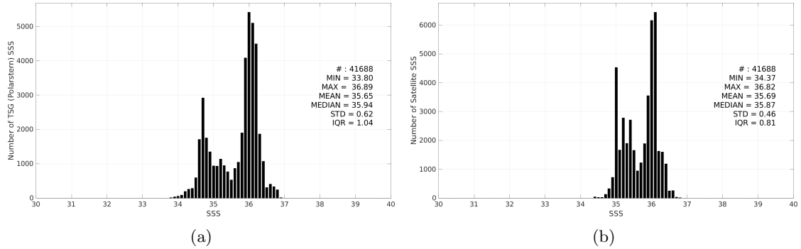
Figure 3: Histograms of SSS from TSG (Polarstern) (a) and SMOS SSS L4 v2 - Daily (BEC) (b) considering all match-up pairs per bins of 0.1 over the Equatorial Ocean 10N-10S Pi-MEP region and for the full satellite product period.
