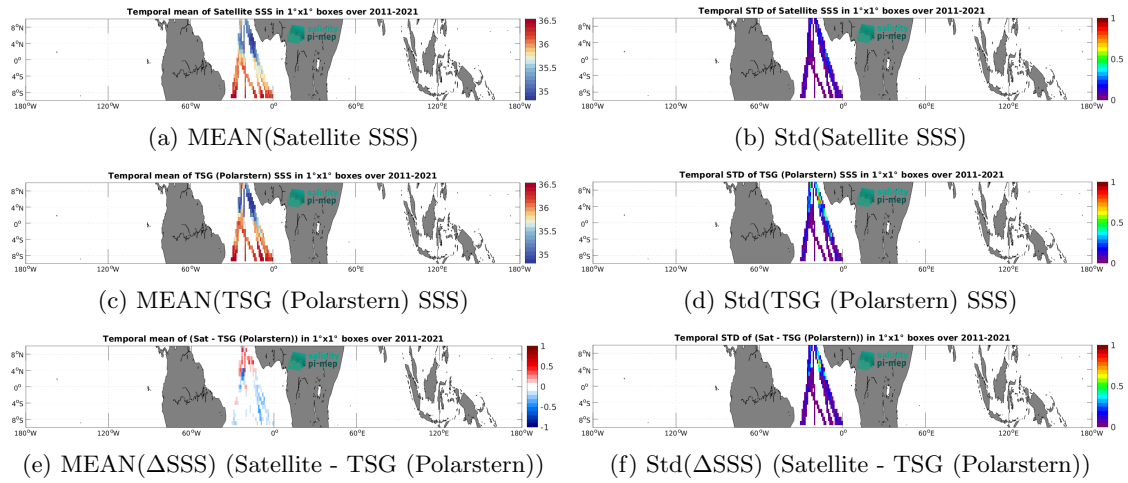
Figure 7: Temporal mean (left) and Std (right) of SSS from SMOS SSS L4 v2 - Daily (BEC) (top), TSG (Polarstern) (middle), and of \Delta SSS (Satellite - TSG (Polarstern)). Only match-up pairs are used to generate these maps.
