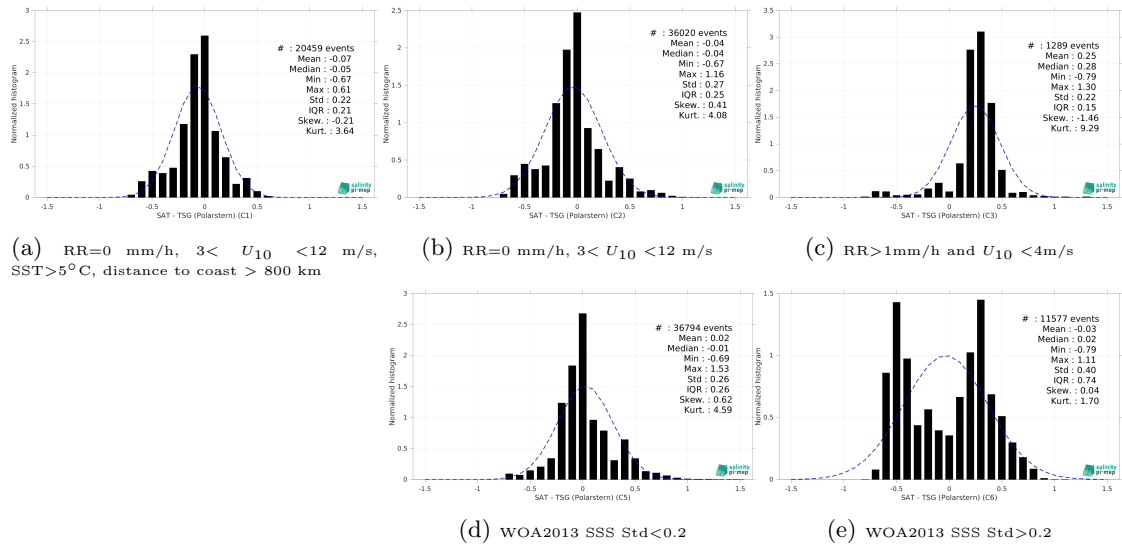
Figure 13: Normalized histogram of \Delta\text{SSS} (SMOS SSS L4 v2 - Daily (BEC) - TSG (Polarstern)) for 5 different subdatasets corresponding to: RR=0 mm/h, 3 < U_{10} < 12 m/s, \text{SST} > 5^\circ\text{C} , distance to coast > 800 km (a), RR=0 mm/h, 3 < U_{10} < 12 m/s (b), RR>1mm/h and U_{10} < 4 m/s (c), WOA2013 SSS Std<0.2 (d), WOA2013 SSS Std>0.2 (e).
