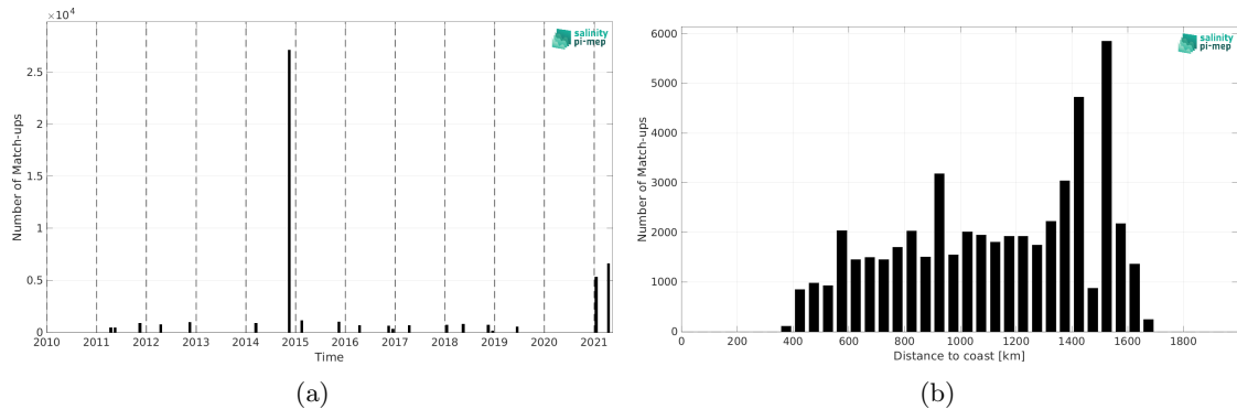
Figure 1: Number of match-ups between TSG (Polarstern) and SMOS SSS L4 v2 - Daily (BEC) SSS as a function of time (a) and as function of the distance to coast (b) over the Equatorial Ocean 10N-10S Pi-MEP region and for the full satellite product period.
