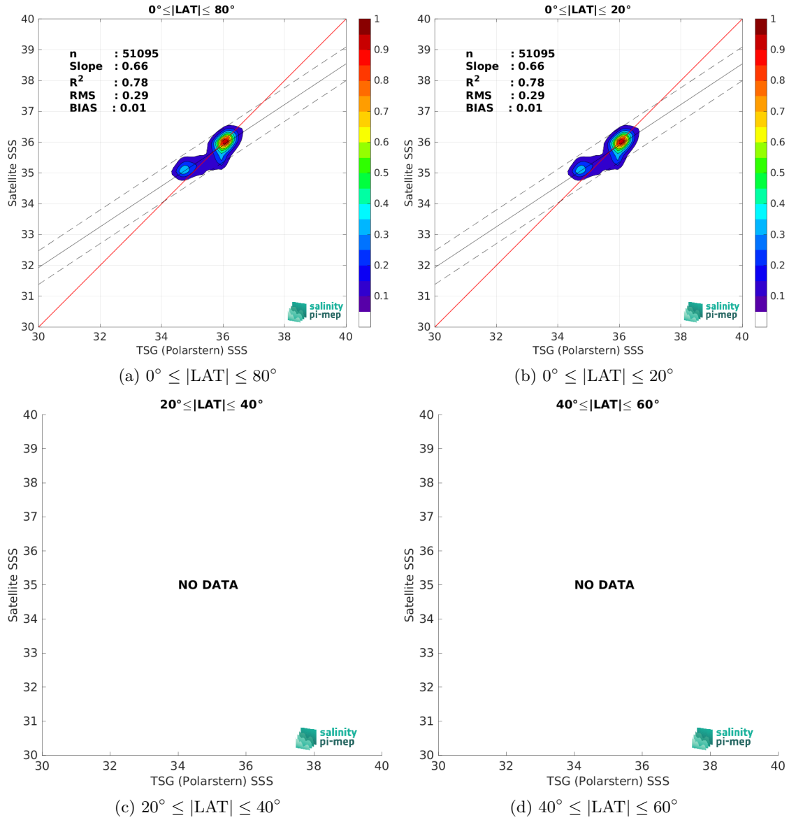
Figure 9: Contour maps of the concentration of SMOS SSS L4 v2 - Daily (BEC) SSS (y-axis) versus TSG (Polarstern) SSS (x-axis) at match-up pairs for different latitude bands. For each plot, the red line shows x=y . The black thin and dashed lines indicate a linear fit through the data cloud and the \pm 95\% confidence levels, respectively. The number match-up pairs n , the slope and R^2 coefficient of the linear fit, the root mean square (RMS) and the mean bias between satellite and in situ data are indicated for each latitude band in each plots.
