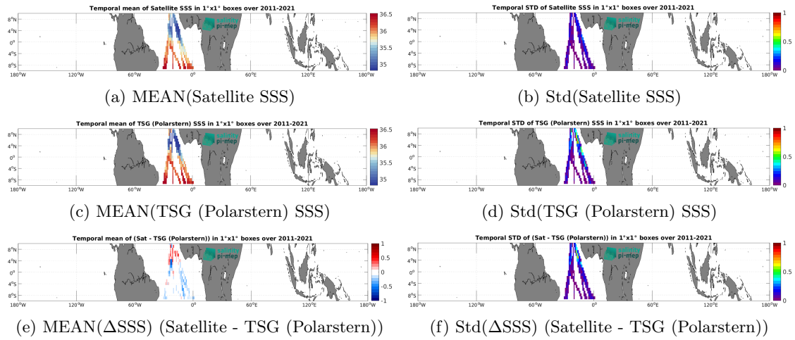
Figure 6: Temporal mean (left) and Std (right) of SSS from SMOS SSS L4 v2 - Daily (BEC) (top), TSG (Polarstern) (middle), and of \Delta SSS (Satellite - TSG (Polarstern)). Only match-up pairs are used to generate these maps.
