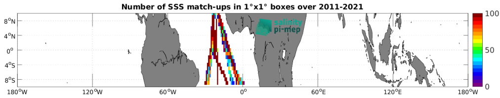
Figure 4: Number of SSS match-ups between TSG (Polarstern) SSS and the SMOS SSS L4 v2 - Daily (BEC) SSS product for the Equatorial Ocean 10N-10S Pi-MEP region over 1^\circ \times 1^\circ boxes and for the full satellite product period.
