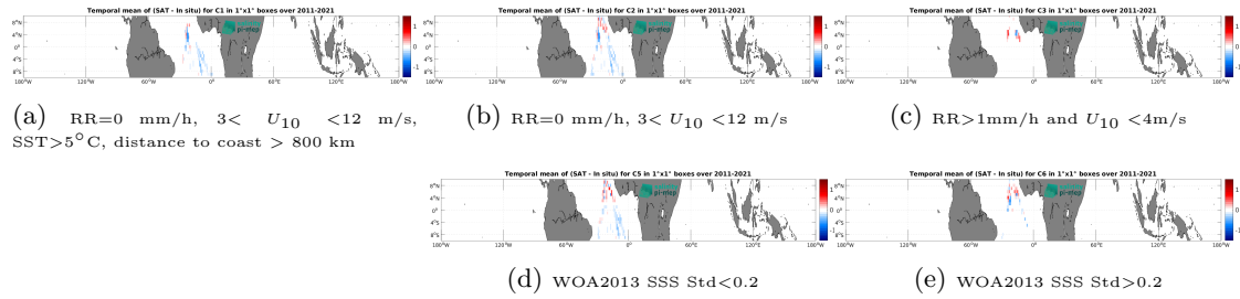
Figure 12: Temporal mean gridded over spatial boxes of size 1^\circ \times 1^\circ of \Delta\text{SSS} (SMOS SSS L4 v2 - Daily (BEC) - TSG (Polarstern)) for 5 different subdatasets corresponding to:RR=0 mm/h, 3 < U_{10} < 12 m/s, \text{SST} > 5^\circ\text{C} , distance to coast > 800 km (a), RR=0 mm/h, 3 < U_{10} < 12 m/s (b), RR>1mm/h and U_{10} < 4 m/s (c), WOA2013 SSS Std<0.2 (d), WOA2013 SSS Std>0.2 (e).
