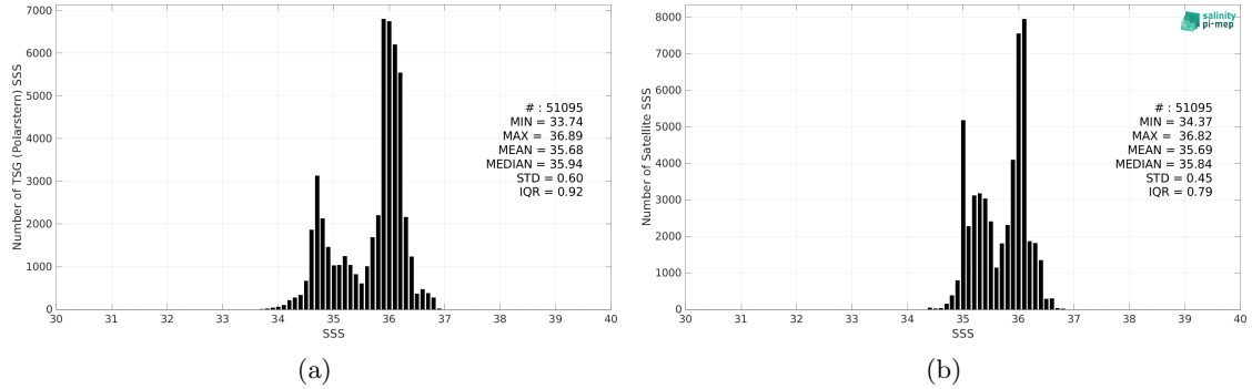
Figure 2: Histograms of SSS from TSG (Polarstern) (a) and SMOS SSS L4 v2 - Daily (BEC) (b) considering all match-up pairs per bins of 0.1 over the Equatorial Ocean 10N-10S Pi-MEP region and for the full satellite product period.
