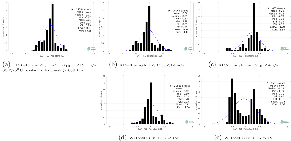
Figure 13: Normalized histogram of \Delta SSS (SMOS SSS L4 v2 - Daily (BEC) - TSG (Polarstern)) for 5 different subdatasets corresponding to: RR=0 mm/h, 3 < U_{10} < 12 m/s, SST > 5^\circ C , distance to coast > 800 km (a), RR=0 mm/h, 3 < U_{10} < 12 m/s (b), RR>1mm/h and U_{10} < 4 m/s (c), WOA2013 SSS Std<0.2 (d), WOA2013 SSS Std>0.2 (e).
