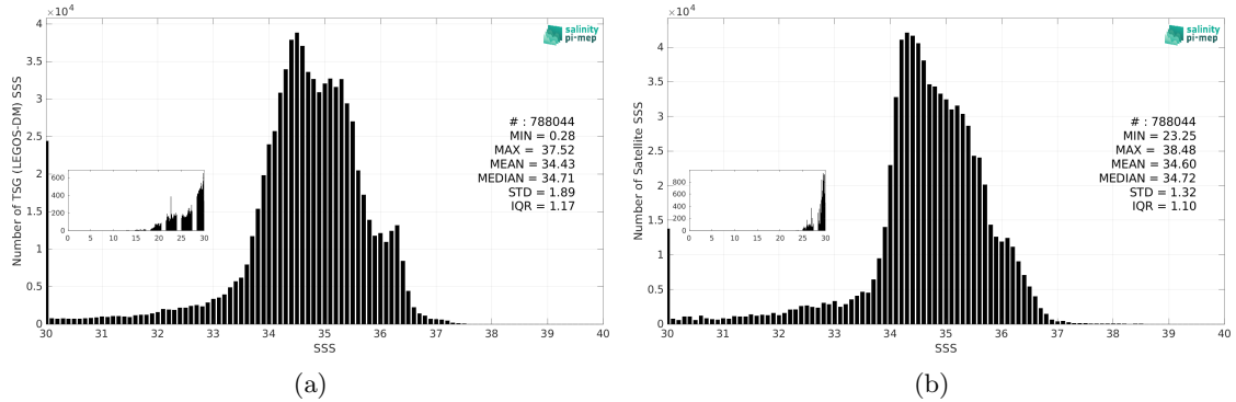
Figure 3: Histograms of SSS from TSG (LEGOS-DM) (a) and SMOS SSS L4 v2 - Daily (BEC) (b) considering all match-up pairs per bins of 0.1 over the Equatorial Ocean 10N-10S Pi-MEP region and for the full satellite product period.
