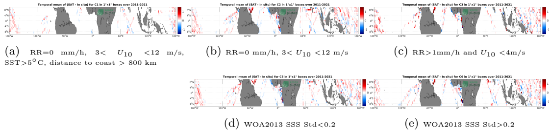
Figure 12: Temporal mean gridded over spatial boxes of size 1^\circ \times 1^\circ of \Delta SSS (SMOS SSS L4 v2 - Daily (BEC) - TSG (LEGOS-DM)) for 5 different subdatasets corresponding to:RR=0 mm/h, 3 < U_{10} < 12 m/s, SST>5°C, distance to coast > 800 km (a), RR=0 mm/h, 3 < U_{10} < 12 m/s (b), RR>1mm/h and U_{10} < 4 m/s (c), WOA2013 SSS Std<0.2 (d), WOA2013 SSS Std>0.2 (e).
