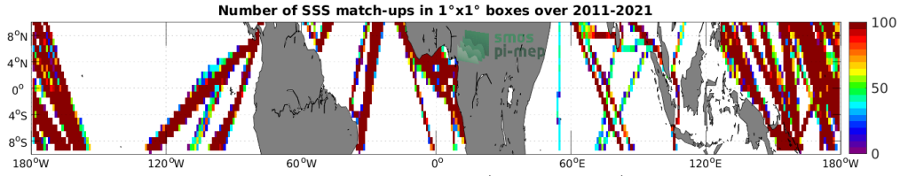
Figure 4: Number of SSS match-ups between TSG (LEGOS-DM) SSS and the SMOS SSS L4 v2 - Daily (BEC) SSS product for the Equatorial Ocean 10N-10S Pi-MEP region over 1^\circ \times 1^\circ boxes and for the full satellite product period.
