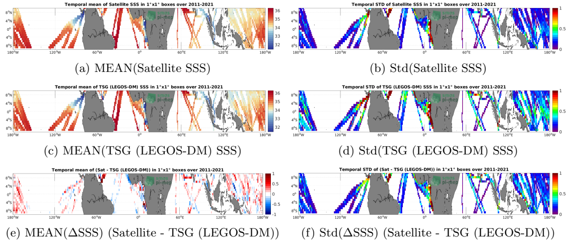
Figure 6: Temporal mean (left) and Std (right) of SSS from SMOS SSS L4 v2 - Daily (BEC) (top), TSG (LEGOS-DM) (middle), and of \Delta SSS (Satellite - TSG (LEGOS-DM)). Only match-up pairs are used to generate these maps.
