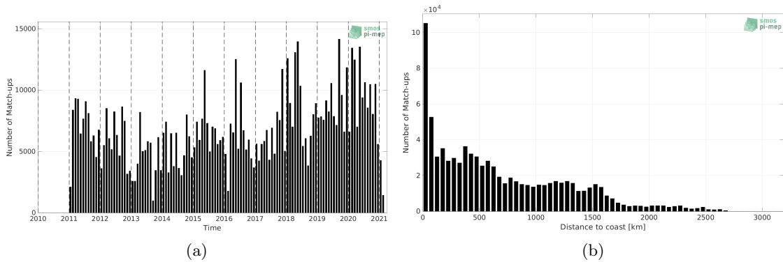
Figure 1: Number of match-ups between TSG (LEGOS-DM) and SMOS SSS L4 v2 - Daily (BEC) SSS as a function of time (a) and as function of the distance to coast (b) over the Equatorial Ocean 10N-10S Pi-MEP region and for the full satellite product period.
