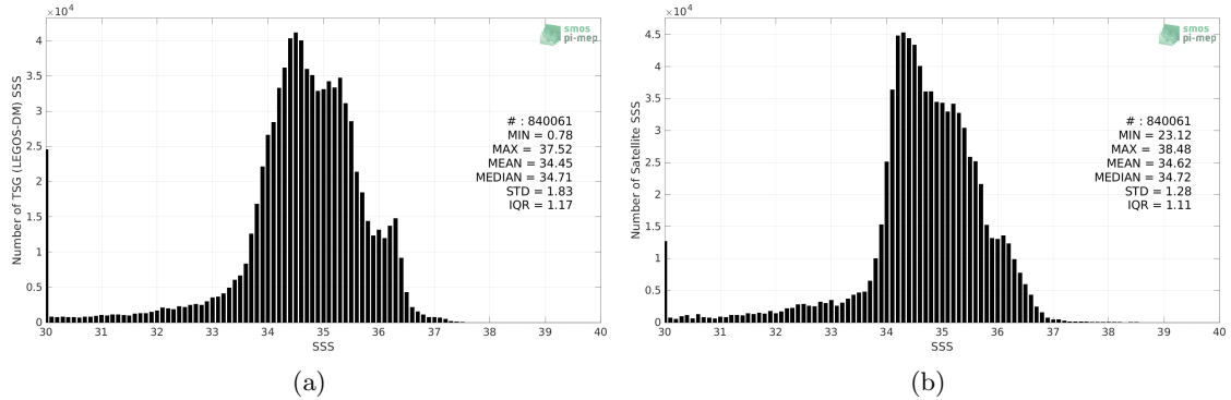
Figure 2: Histograms of SSS from TSG (LEGOS-DM) (a) and SMOS SSS L4 v2 - Daily (BEC) (b) considering all match-up pairs per bins of 0.1 over the Equatorial Ocean 10N-10S Pi-MEP region and for the full satellite product period.
