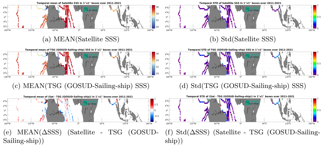
Figure 7: Temporal mean (left) and Std (right) of SSS from SMOS SSS L4 v2 - Daily (BEC) (top), TSG (GOSUD-Sailing-ship) (middle), and of \Delta SSS (Satellite - TSG (GOSUD-Sailing-ship)). Only match-up pairs are used to generate these maps.
