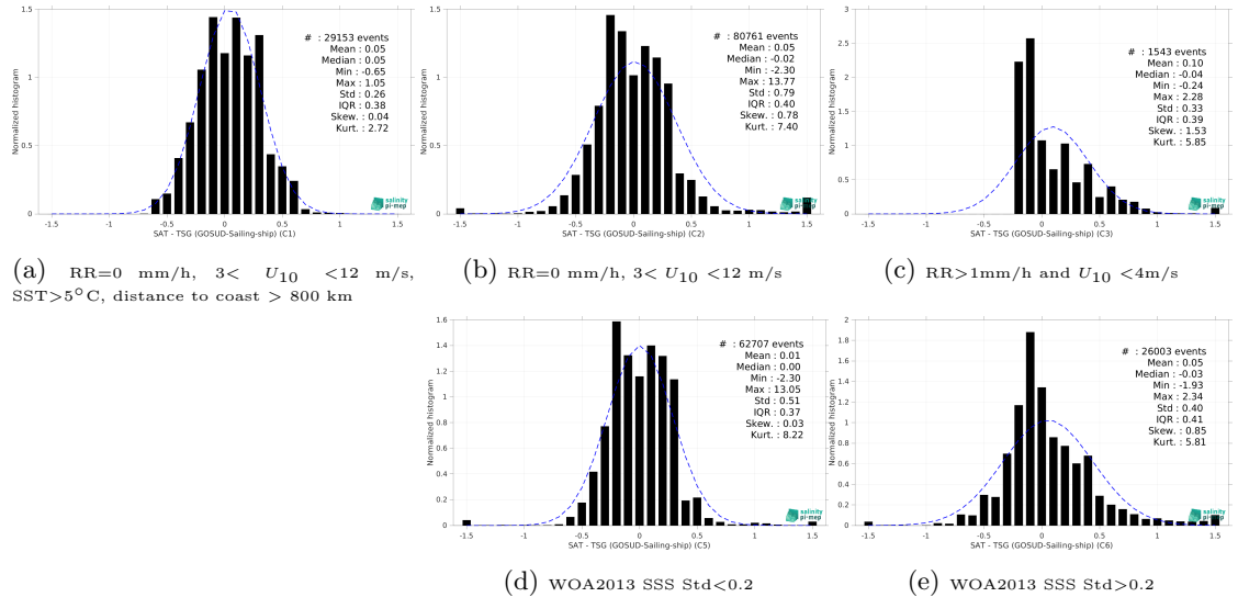
Figure 15: Normalized histogram of \Delta SSS (SMOS SSS L4 v2 - Daily (BEC) - TSG (GOSUD-Sailing-ship)) for 5 different subdatasets corresponding to: RR=0 mm/h, 3 < U_{10} < 12 m/s, SST>5°C, distance to coast > 800 km (a), RR=0 mm/h, 3 < U_{10} < 12 m/s (b), RR>1mm/h and U_{10} < 4 m/s (c), WOA2013 SSS Std<0.2 (d), WOA2013 SSS Std>0.2 (e).
