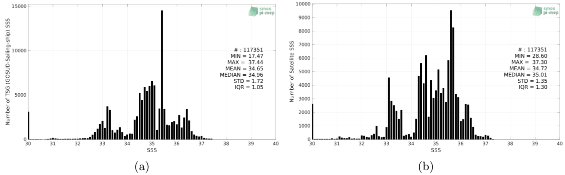
Figure 2: Histograms of SSS from TSG (GOSUD-Sailing-ship) (a) and SMOS SSS L4 v2 - Daily (BEC) (b) considering all match-up pairs per bins of 0.1 over the Equatorial Ocean 10N-10S Pi-MEP region and for the full satellite product period.
