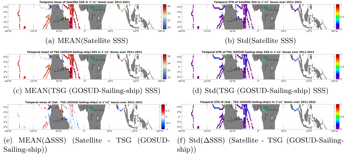
Figure 6: Temporal mean (left) and Std (right) of SSS from SMOS SSS L4 v2 - Daily (BEC) (top), TSG (GOSUD-Sailing-ship) (middle), and of \Delta SSS (Satellite - TSG (GOSUD-Sailing-ship)). Only match-up pairs are used to generate these maps.
