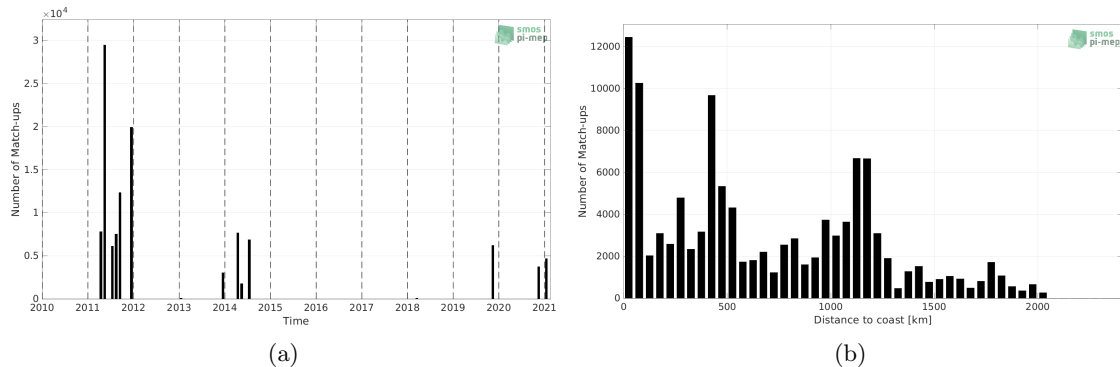
Figure 1: Number of match-ups between TSG (GOSUD-Sailing-ship) and SMOS SSS L4 v2 - Daily (BEC) SSS as a function of time (a) and as function of the distance to coast (b) over the Equatorial Ocean 10N-10S Pi-MEP region and for the full satellite product period.
