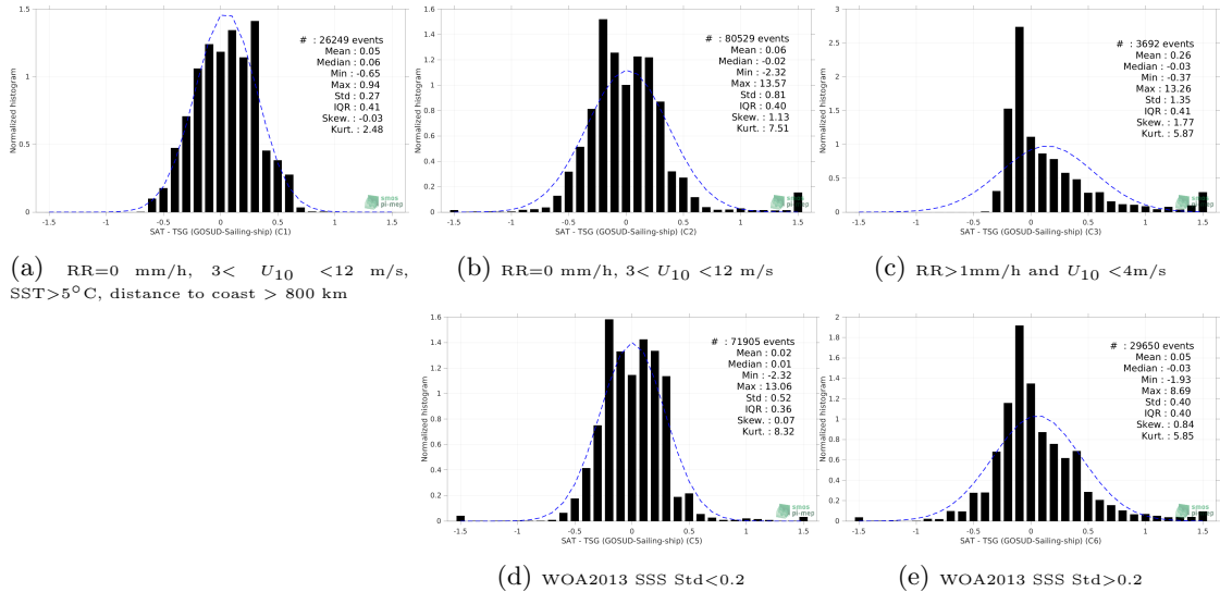
Figure 13: Normalized histogram of \Delta SSS (SMOS SSS L4 v2 - Daily (BEC) - TSG (GOSUD-Sailing-ship)) for 5 different subdatasets corresponding to: RR=0 mm/h, 3 < U_{10} < 12 m/s, SST> 5^\circ\text{C} , distance to coast > 800 km (a), RR=0 mm/h, 3 < U_{10} < 12 m/s (b), RR>1mm/h and U_{10} < 4 m/s (c), WOA2013 SSS Std<0.2 (d), WOA2013 SSS Std>0.2 (e).
