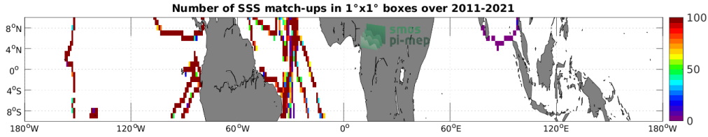
Figure 4: Number of SSS match-ups between TSG (GOSUD-Sailing-ship) SSS and the SMOS SSS L4 v2 - Daily (BEC) SSS product for the Equatorial Ocean 10N-10S Pi-MEP region over 1^\circ \times 1^\circ boxes and for the full satellite product period.
