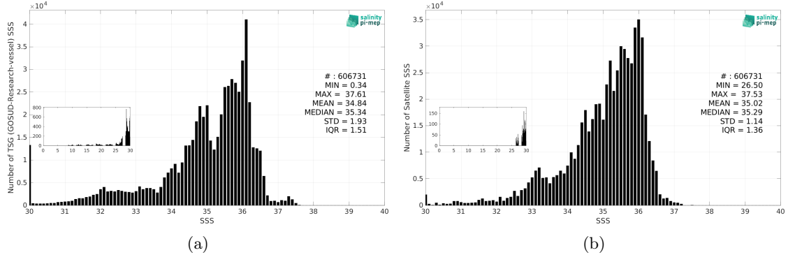
Figure 3: Histograms of SSS from TSG (GOSUD-Research-vessel) (a) and SMOS SSS L4 v2 - Daily (BEC) (b) considering all match-up pairs per bins of 0.1 over the Equatorial Ocean 10N-10S Pi-MEP region and for the full satellite product period.
