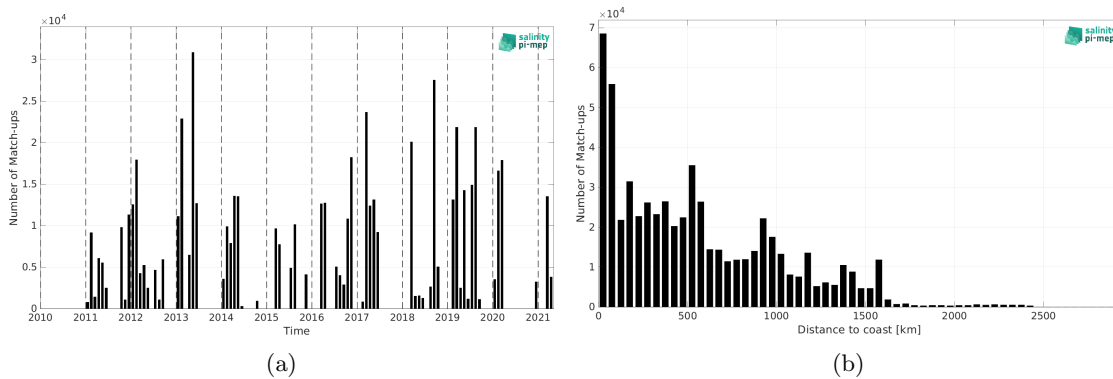
Figure 2: Number of match-ups between TSG (GOSUD-Research-vessel) and SMOS SSS L4 v2 - Daily (BEC) SSS as a function of time (a) and as function of the distance to coast (b) over the Equatorial Ocean 10N-10S Pi-MEP region and for the full satellite product period.
