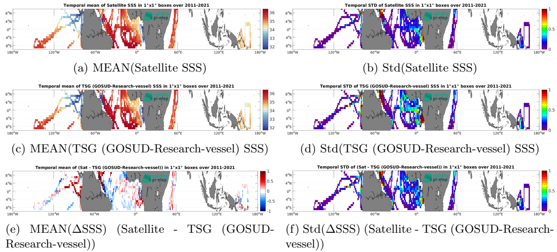
Figure 7: Temporal mean (left) and Std (right) of SSS from SMOS SSS L4 v2 - Daily (BEC) (top), TSG (GOSUD-Research-vessel) (middle), and of \Delta SSS (Satellite - TSG (GOSUD-Research-vessel)). Only match-up pairs are used to generate these maps.
