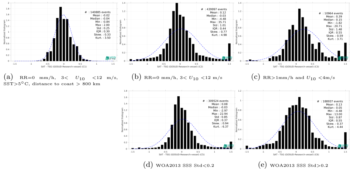
Figure 15: Normalized histogram of \Delta SSS (SMOS SSS L4 v2 - Daily (BEC) - TSG (GOSUD-Research-vessel)) for 5 different subdatasets corresponding to: RR=0 mm/h, 3 < U_{10} < 12 m/s, SST >5^\circ C, distance to coast > 800 km (a), RR=0 mm/h, 3 < U_{10} < 12 m/s (b), RR >1 mm/h and U_{10} < 4 m/s (c), WOA2013 SSS Std <0.2 (d), WOA2013 SSS Std >0.2 (e).
