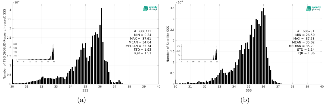
Figure 3: Histograms of SSS from TSG (GOSUD-Research-vessel) (a) and SMOS SSS L4 v2 - Daily (BEC) (b) considering all match-up pairs per bins of 0.1 over the Equatorial Ocean 10N-10S Pi-MEP region and for the full satellite product period.
