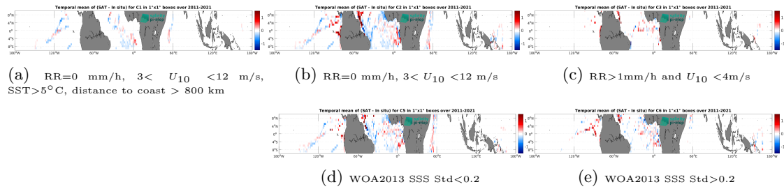
Figure 14: Temporal mean gridded over spatial boxes of size 1^\circ \times 1^\circ of \Delta SSS (SMOS SSS L4 v2 - Daily (BEC) - TSG (GOSUD-Research-vessel)) for 5 different subdatasets corresponding to: RR=0 mm/h, 3 < U_{10} < 12 m/s, SST >5^\circ C, distance to coast > 800 km (a), RR=0 mm/h, 3 < U_{10} < 12 m/s (b), RR >1 mm/h and U_{10} < 4 m/s (c), WOA2013 SSS Std <0.2 (d), WOA2013 SSS Std >0.2 (e).
