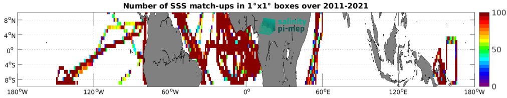
Figure 5: Number of SSS match-ups between TSG (GOSUD-Research-vessel) SSS and the SMOS SSS L4 v2 - Daily (BEC) SSS product for the Equatorial Ocean 10N-10S Pi-MEP region over 1^\circ \times 1^\circ boxes and for the full satellite product period.
