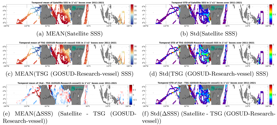
Figure 6: Temporal mean (left) and Std (right) of SSS from SMOS SSS L4 v2 - Daily (BEC) (top), TSG (GOSUD-Research-vessel) (middle), and of \Delta SSS (Satellite - TSG (GOSUD-Research-vessel)). Only match-up pairs are used to generate these maps.
