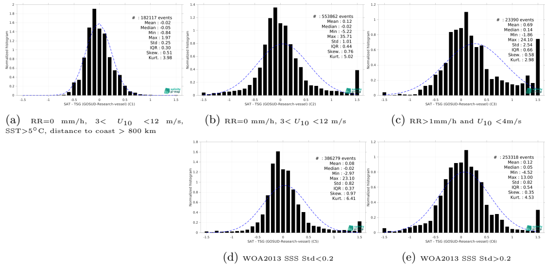
Figure 13: Normalized histogram of \Delta SSS (SMOS SSS L4 v2 - Daily (BEC) - TSG (GOSUD-Research-vessel)) for 5 different subdatasets corresponding to: RR=0 mm/h, 3 < U_{10} < 12 m/s, SST> 5^\circ\text{C} , distance to coast > 800 km (a), RR=0 mm/h, 3 < U_{10} < 12 m/s (b), RR>1mm/h and U_{10} < 4 m/s (c), WOA2013 SSS Std<0.2 (d), WOA2013 SSS Std>0.2 (e).
