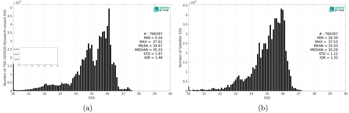
Figure 2: Histograms of SSS from TSG (GOSUD-Research-vessel) (a) and SMOS SSS L4 v2 - Daily (BEC) (b) considering all match-up pairs per bins of 0.1 over the Equatorial Ocean 10N-10S Pi-MEP region and for the full satellite product period.
