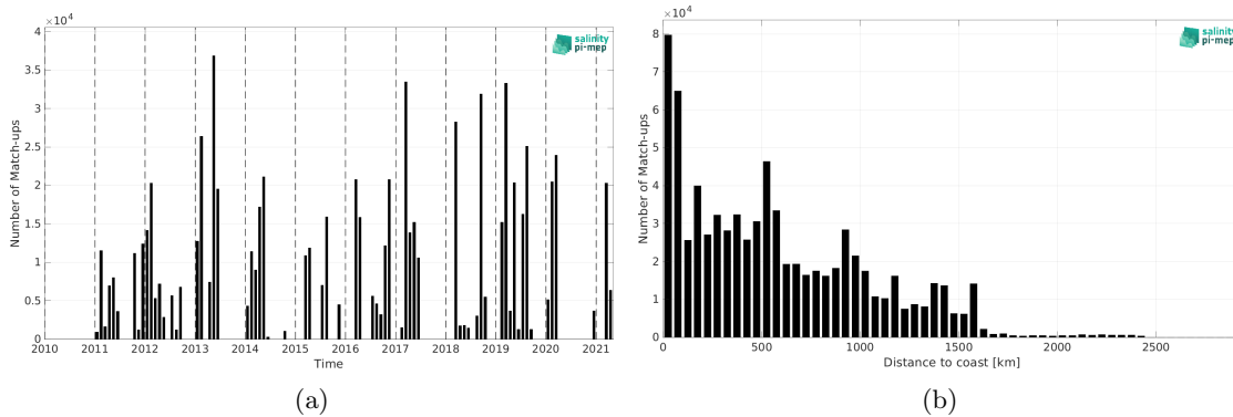
Figure 1: Number of match-ups between TSG (GOSUD-Research-vessel) and SMOS SSS L4 v2 - Daily (BEC) SSS as a function of time (a) and as function of the distance to coast (b) over the Equatorial Ocean 10N-10S Pi-MEP region and for the full satellite product period.
