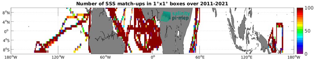
Figure 4: Number of SSS match-ups between TSG (GOSUD-Research-vessel) SSS and the SMOS SSS L4 v2 - Daily (BEC) SSS product for the Equatorial Ocean 10N-10S Pi-MEP region over 1^\circ \times 1^\circ boxes and for the full satellite product period.
