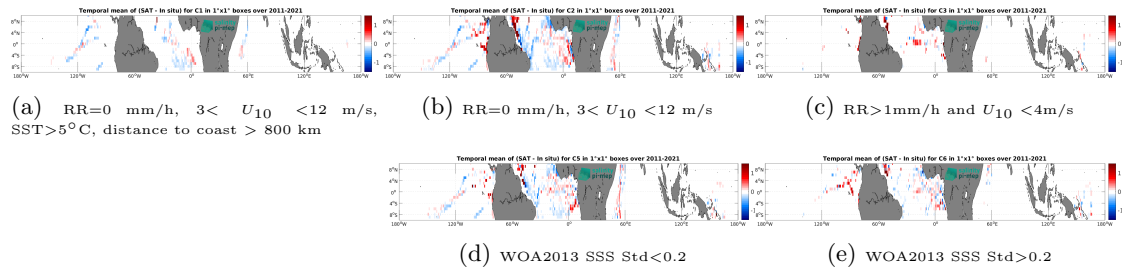
Figure 12: Temporal mean gridded over spatial boxes of size 1^\circ \times 1^\circ of \Delta SSS (SMOS SSS L4 v2 - Daily (BEC) - TSG (GOSUD-Research-vessel)) for 5 different subdatasets corresponding to: RR=0 mm/h, 3 < U_{10} < 12 m/s, SST> 5^\circ\text{C} , distance to coast > 800 km (a), RR=0 mm/h, 3 < U_{10} < 12 m/s (b), RR>1mm/h and U_{10} < 4 m/s (c), WOA2013 SSS Std<0.2 (d), WOA2013 SSS Std>0.2 (e).
