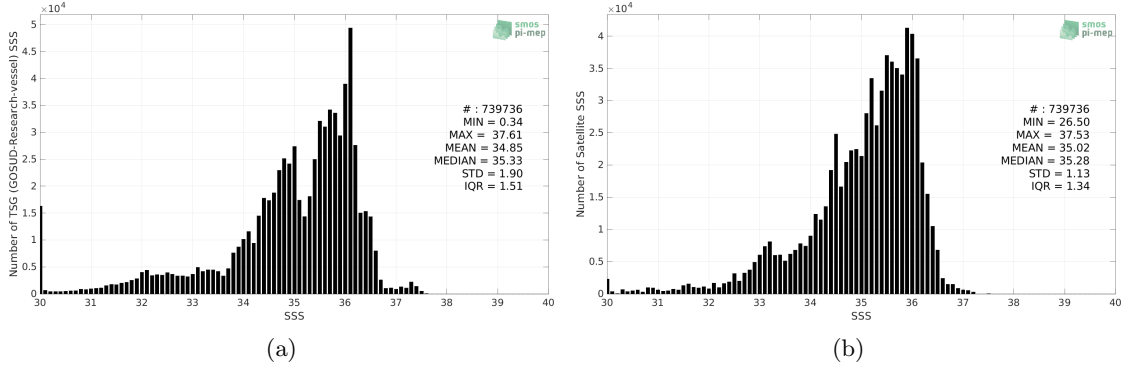
Figure 2: Histograms of SSS from TSG (GOSUD-Research-vessel) (a) and SMOS SSS L4 v2 - Daily (BEC) (b) considering all match-up pairs per bins of 0.1 over the Equatorial Ocean 10N-10S Pi-MEP region and for the full satellite product period.
