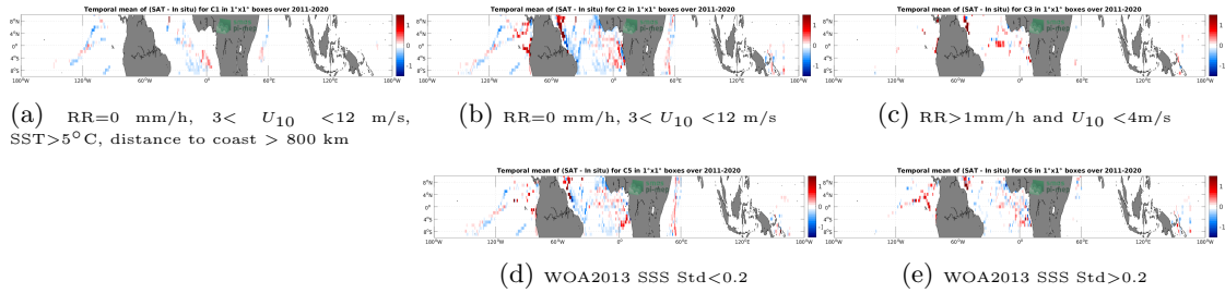
Figure 12: Temporal mean gridded over spatial boxes of size 1^\circ \times 1^\circ of \Delta SSS (SMOS SSS L4 v2 - Daily (BEC) - TSG (GOSUD-Research-vessel)) for 5 different subdatasets corresponding to: RR=0 mm/h, 3 < U_{10} < 12 m/s, SST>5°C, distance to coast > 800 km (a), RR=0 mm/h, 3 < U_{10} < 12 m/s (b), RR>1mm/h and U_{10} < 4 m/s (c), WOA2013 SSS Std<0.2 (d), WOA2013 SSS Std>0.2 (e).
