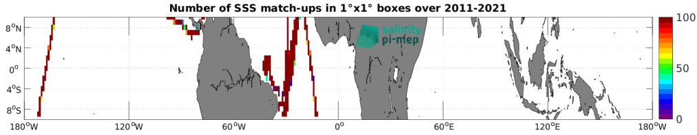
Figure 5: Number of SSS match-ups between TSG (CSIC-UTM) SSS and the SMOS SSS L4 v2 - Daily (BEC) SSS product for the Equatorial Ocean 10N-10S Pi-MEP region over 1^\circ \times 1^\circ boxes and for the full satellite product period.
