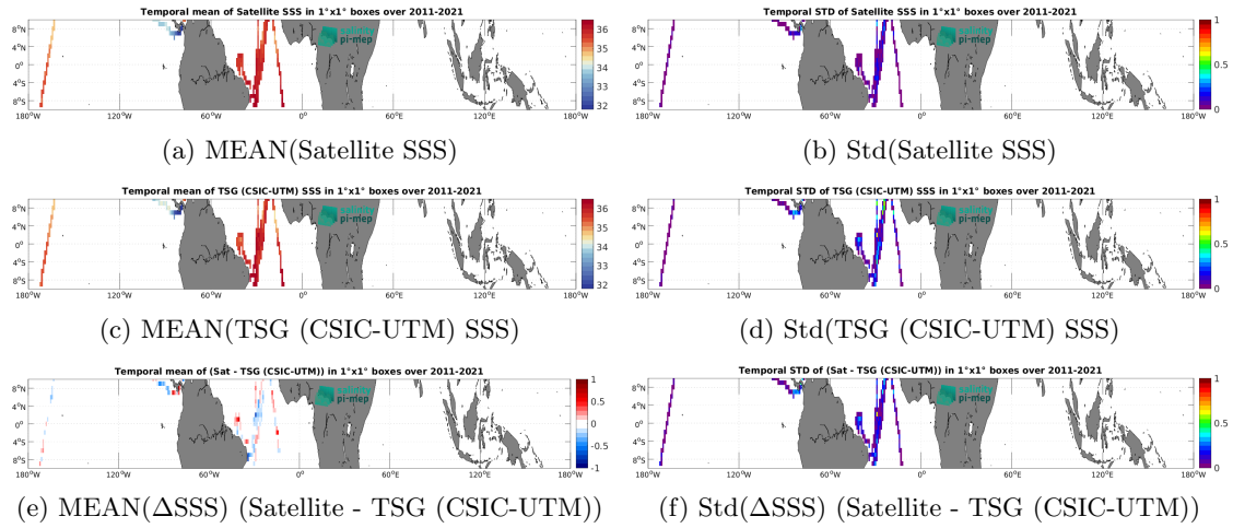
Figure 7: Temporal mean (left) and Std (right) of SSS from SMOS SSS L4 v2 - Daily (BEC) (top), TSG (CSIC-UTM) (middle), and of \Delta SSS (Satellite - TSG (CSIC-UTM)). Only match-up pairs are used to generate these maps.
