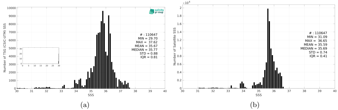
Figure 3: Histograms of SSS from TSG (CSIC-UTM) (a) and SMOS SSS L4 v2 - Daily (BEC) (b) considering all match-up pairs per bins of 0.1 over the Equatorial Ocean 10N-10S Pi-MEP region and for the full satellite product period.
