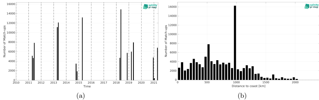
Figure 2: Number of match-ups between TSG (CSIC-UTM) and SMOS SSS L4 v2 - Daily (BEC) SSS as a function of time (a) and as function of the distance to coast (b) over the Equatorial Ocean 10N-10S Pi-MEP region and for the full satellite product period.
