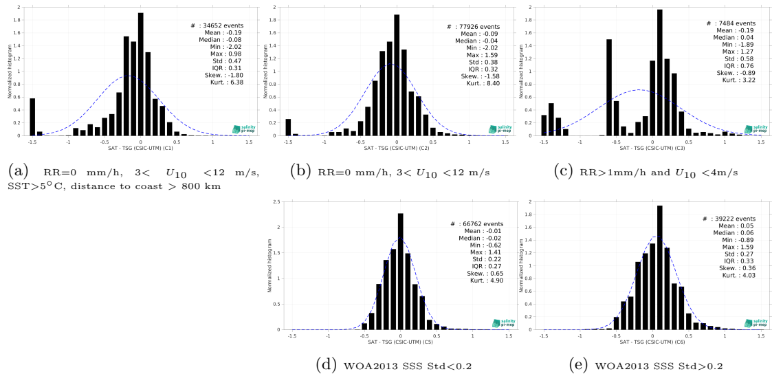
Figure 13: Normalized histogram of \Delta SSS (SMOS SSS L4 v2 - Daily (BEC) - TSG (CSIC-UTM)) for 5 different subdatasets corresponding to: RR=0 mm/h, 3 < U_{10} < 12 m/s, SST >5^\circ C, distance to coast > 800 km (a), RR=0 mm/h, 3 < U_{10} < 12 m/s (b), RR >1 mm/h and U_{10} < 4 m/s (c), WOA2013 SSS Std <0.2 (d), WOA2013 SSS Std >0.2 (e).
