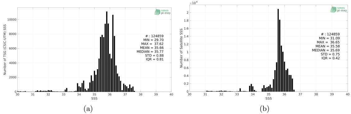
Figure 2: Histograms of SSS from TSG (CSIC-UTM) (a) and SMOS SSS L4 v2 - Daily (BEC) (b) considering all match-up pairs per bins of 0.1 over the Equatorial Ocean 10N-10S Pi-MEP region and for the full satellite product period.
