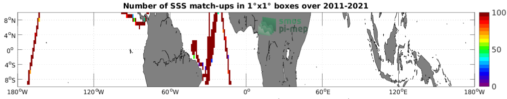
Figure 4: Number of SSS match-ups between TSG (CSIC-UTM) SSS and the SMOS SSS L4 v2 - Daily (BEC) SSS product for the Equatorial Ocean 10N-10S Pi-MEP region over 1^\circ \times 1^\circ boxes and for the full satellite product period.
