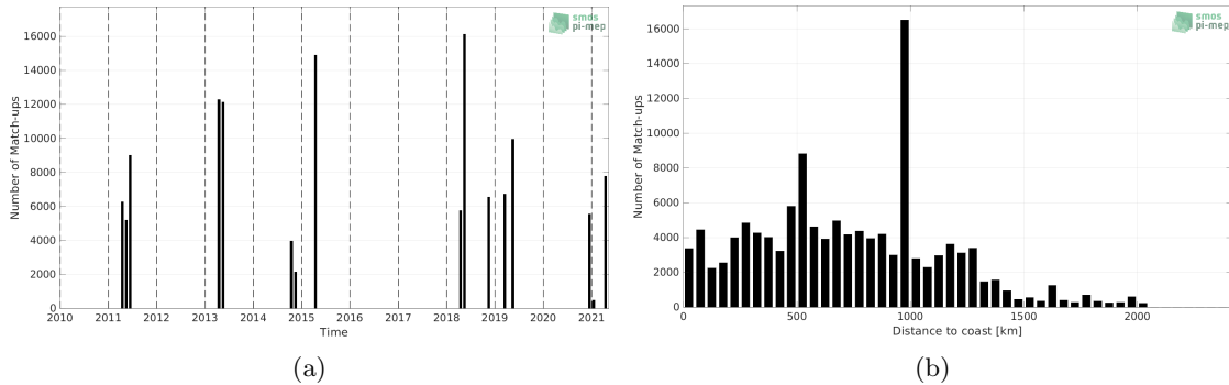
Figure 1: Number of match-ups between TSG (CSIC-UTM) and SMOS SSS L4 v2 - Daily (BEC) SSS as a function of time (a) and as function of the distance to coast (b) over the Equatorial Ocean 10N-10S Pi-MEP region and for the full satellite product period.
