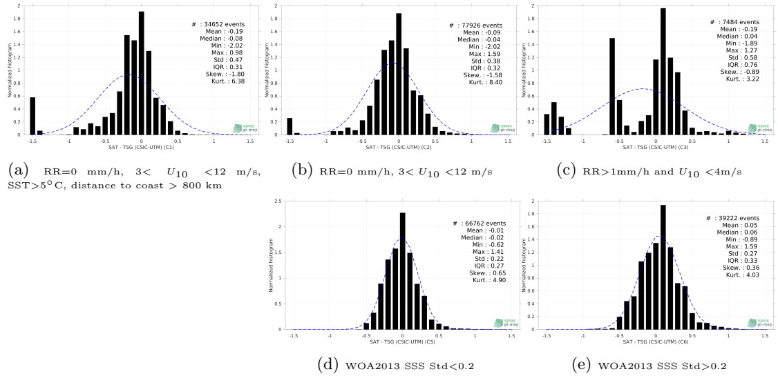
Figure 13: Normalized histogram of \Delta SSS (SMOS SSS L4 v2 - Daily (BEC) - TSG (CSIC-UTM)) for 5 different subdatasets corresponding to: RR=0 mm/h, 3 < U_{10} < 12 m/s, SST >5^\circ\text{C} , distance to coast > 800 km (a), RR=0 mm/h, 3 < U_{10} < 12 m/s (b), RR >1 mm/h and U_{10} < 4 m/s (c), WOA2013 SSS Std <0.2 (d), WOA2013 SSS Std >0.2 (e).
