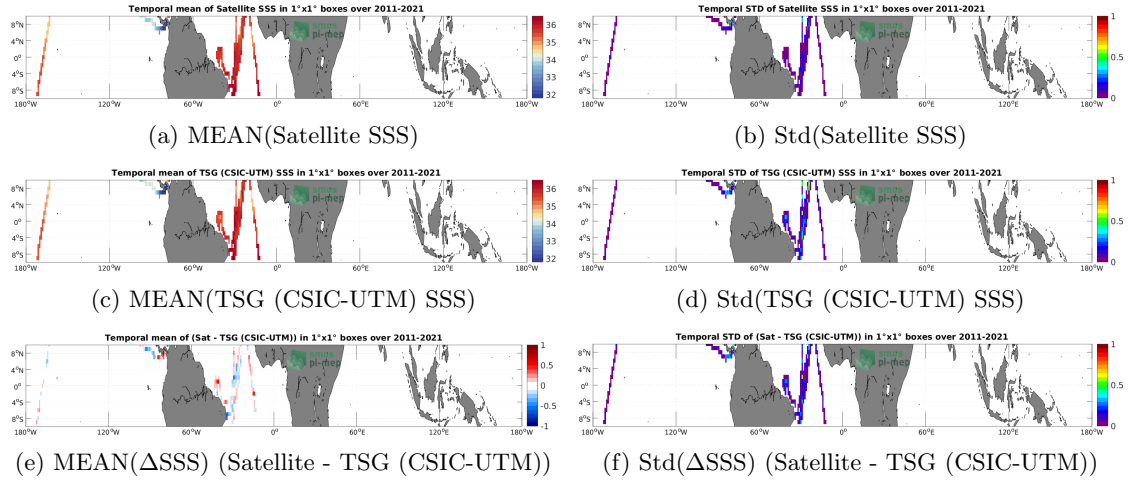
Figure 6: Temporal mean (left) and Std (right) of SSS from SMOS SSS L4 v2 - Daily (BEC) (top), TSG (CSIC-UTM) (middle), and of \Delta SSS (Satellite - TSG (CSIC-UTM)). Only match-up pairs are used to generate these maps.
