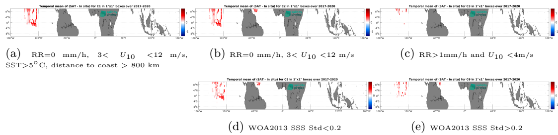
Figure 14: Temporal mean gridded over spatial boxes of size 1^\circ \times 1^\circ of \Delta\text{SSS} (SMOS SSS L4 v2 - Daily (BEC) - Saildrone) for 5 different subdatasets corresponding to: RR=0 mm/h, 3 < U_{10} < 12 m/s, SST>5°C, distance to coast > 800 km (a), RR=0 mm/h, 3 < U_{10} < 12 m/s (b), RR>1mm/h and U_{10} < 4 m/s (c), WOA2013 SSS Std<0.2 (d), WOA2013 SSS Std>0.2 (e).
