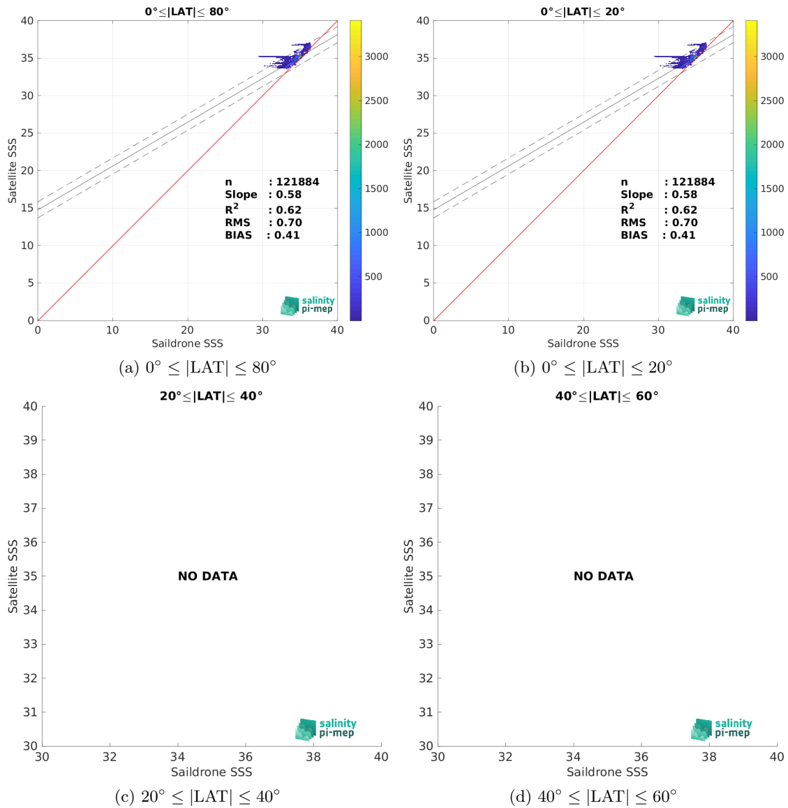
Figure 10: Contour maps of the concentration of SMOS SSS L4 v2 - Daily (BEC) SSS (y-axis) versus Sairdrone SSS (x-axis) at match-up pairs for different latitude bands. For each plot, the red line shows x=y . The black thin and dashed lines indicate a linear fit through the data cloud and the \pm 95\% confidence levels, respectively. The number match-up pairs n , the slope and R^2 coefficient of the linear fit, the root mean square (RMS) and the mean bias between satellite and in situ data are indicated for each latitude band in each plots.
