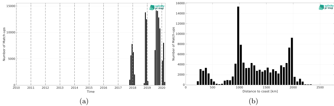
Figure 2: Number of match-ups between Saildrone and SMOS SSS L4 v2 - Daily (BEC) SSS as a function of time (a) and as function of the distance to coast (b) over the Equatorial Ocean 10N-10S Pi-MEP region and for the full satellite product period.
