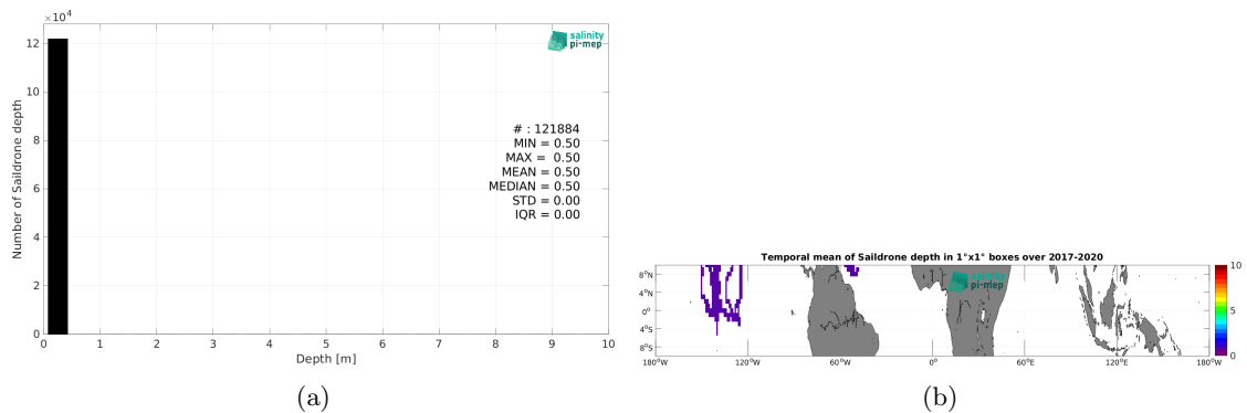
Figure 4: Histograms of the depth of the upper level SSS measurements from Sairdrone in the Match-up DataBase for the Equatorial Ocean 10N-10S Pi-MEP region (a) and temporal mean spatial distribution of pressure of the in situ SSS data over 1^\circ \times 1^\circ boxes and for the full satellite product period (b).
