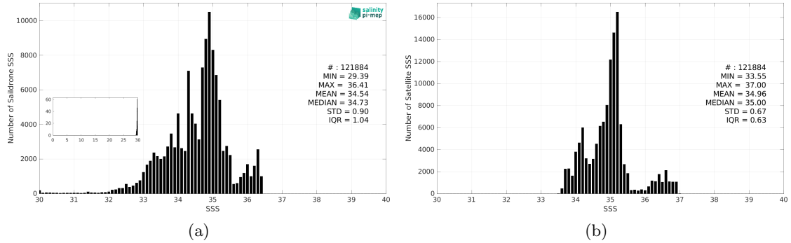
Figure 3: Histograms of SSS from Sairdrone (a) and SMOS SSS L4 v2 - Daily (BEC) (b) considering all match-up pairs per bins of 0.1 over the Equatorial Ocean 10N-10S Pi-MEP region and for the full satellite product period.
