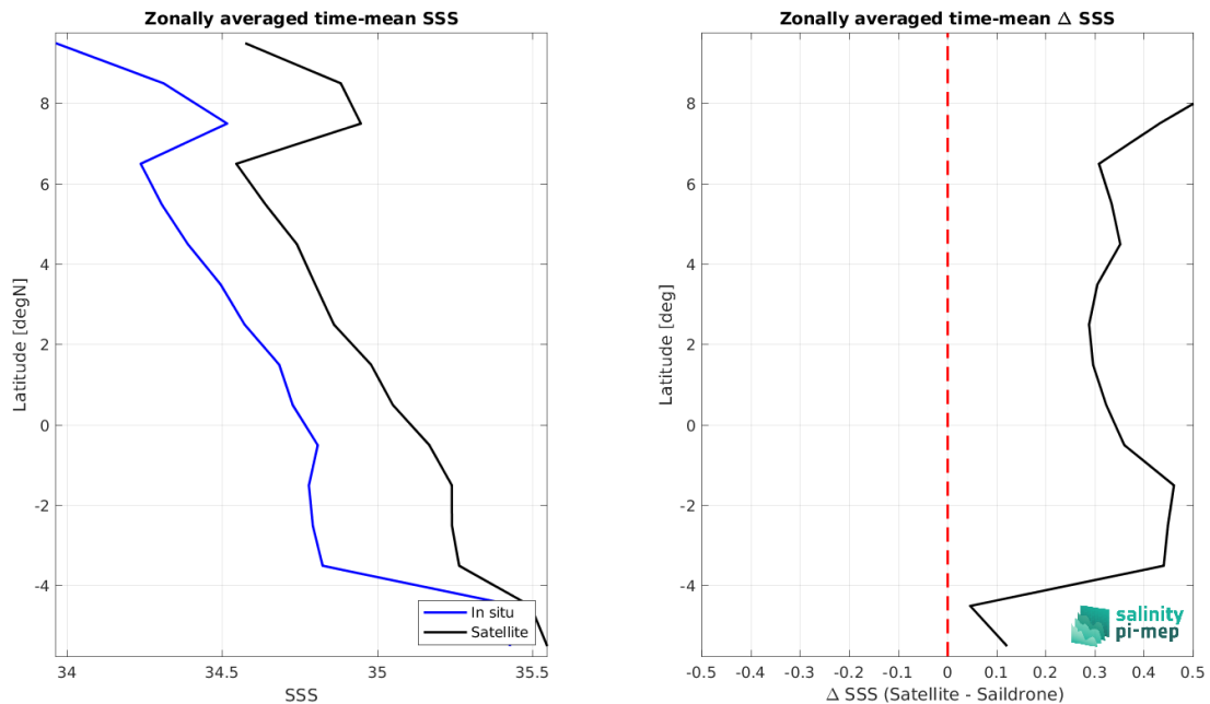
Figure 9: Left panel: Zonal mean SSS from SMOS SSS L4 v2 - Daily (BEC) satellite product (black) and from Sairdrone (blue). Right panel: Zonal mean of \Delta SSS (Satellite - Sairdrone) for all the collected Pi-MEP match-up pairs estimated over the full satellite product period.
