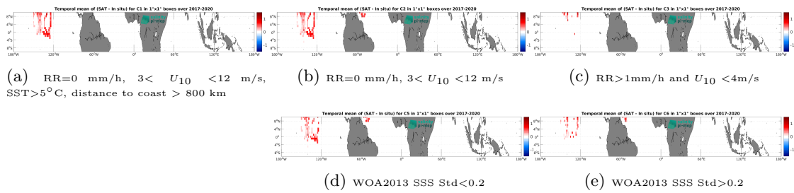
Figure 14: Temporal mean gridded over spatial boxes of size 1^\circ \times 1^\circ of \Delta SSS (SMOS SSS L4 v2 - Daily (BEC) - Saildrone) for 5 different subdatasets corresponding to: RR=0 mm/h, 3 < U_{10} < 12 m/s, SST>5°C, distance to coast > 800 km (a), RR=0 mm/h, 3 < U_{10} < 12 m/s (b), RR>1mm/h and U_{10} < 4 m/s (c), WOA2013 SSS Std<0.2 (d), WOA2013 SSS Std>0.2 (e).
