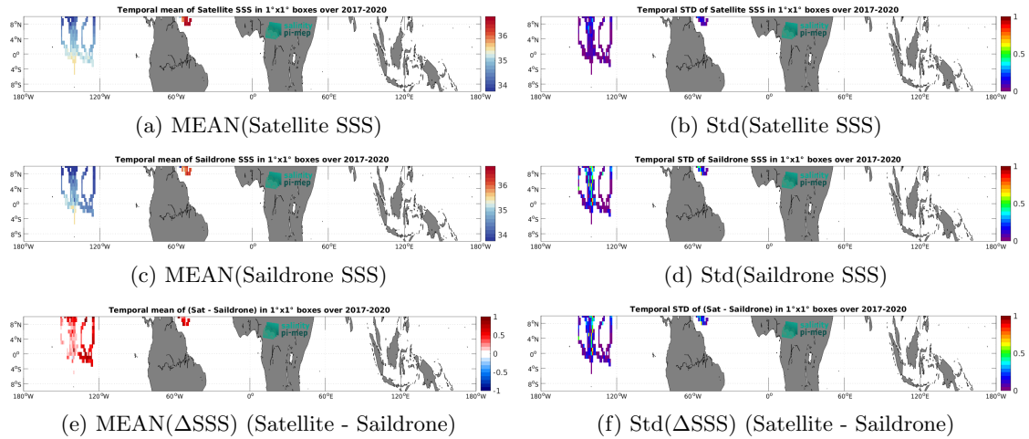
Figure 7: Temporal mean (left) and Std (right) of SSS from SMOS SSS L4 v2 - Daily (BEC) (top), Saildrone (middle), and of \Delta SSS (Satellite - Saildrone). Only match-up pairs are used to generate these maps.
