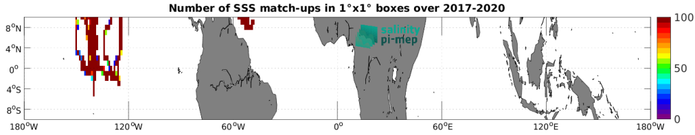
Figure 5: Number of SSS match-ups between Saildrone SSS and the SMOS SSS L4 v2 - Daily (BEC) SSS product for the Equatorial Ocean 10N-10S Pi-MEP region over 1^\circ \times 1^\circ boxes and for the full satellite product period.
