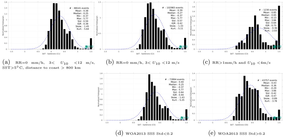
Figure 15: Normalized histogram of \Delta SSS (SMOS SSS L4 v2 - Daily (BEC) - Saildrone) for 5 different subdatasets corresponding to: RR=0 mm/h, 3 < U_{10} < 12 m/s, SST>5°C, distance to coast > 800 km (a), RR=0 mm/h, 3 < U_{10} < 12 m/s (b), RR>1mm/h and U_{10} < 4 m/s (c), WOA2013 SSS Std<0.2 (d), WOA2013 SSS Std>0.2 (e).
