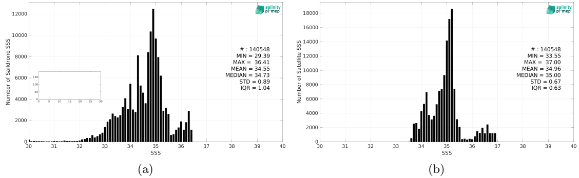
Figure 2: Histograms of SSS from Sairdrone (a) and SMOS SSS L4 v2 - Daily (BEC) (b) considering all match-up pairs per bins of 0.1 over the Equatorial Ocean 10N-10S Pi-MEP region and for the full satellite product period.
