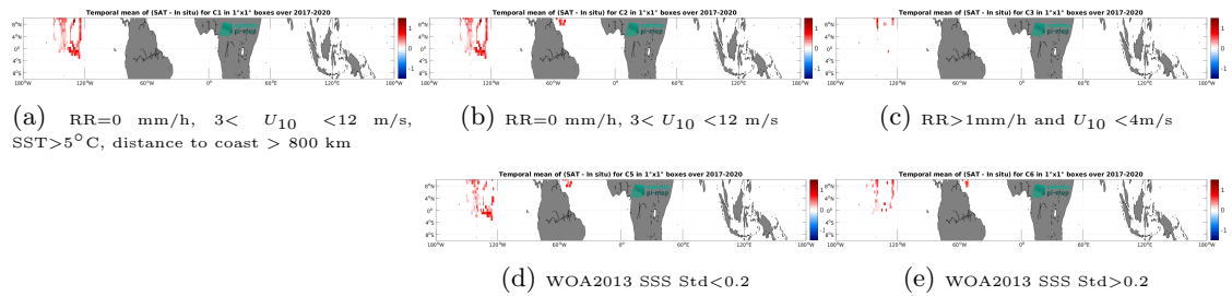
Figure 12: Temporal mean gridded over spatial boxes of size 1^\circ \times 1^\circ of \Delta SSS (SMOS SSS L4 v2 - Daily (BEC) - Saildrone) for 5 different subdatasets corresponding to:RR=0 mm/h, 3 < U_{10} < 12 m/s, SST >5^\circ\text{C} , distance to coast > 800 km (a), RR=0 mm/h, 3 < U_{10} < 12 m/s (b), RR >1 mm/h and U_{10} < 4 m/s (c), WOA2013 SSS Std <0.2 (d), WOA2013 SSS Std >0.2 (e).
