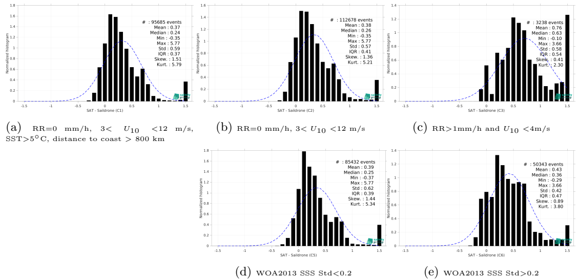
Figure 13: Normalized histogram of \Delta SSS (SMOS SSS L4 v2 - Daily (BEC) - Saildrone) for 5 different subdatasets corresponding to: RR=0 mm/h, 3 < U_{10} < 12 m/s, SST >5^\circ\text{C} , distance to coast > 800 km (a), RR=0 mm/h, 3 < U_{10} < 12 m/s (b), RR >1 mm/h and U_{10} < 4 m/s (c), WOA2013 SSS Std <0.2 (d), WOA2013 SSS Std >0.2 (e).
