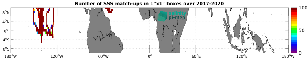
Figure 4: Number of SSS match-ups between Saildrone SSS and the SMOS SSS L4 v2 - Daily (BEC) SSS product for the Equatorial Ocean 10N-10S Pi-MEP region over 1^\circ \times 1^\circ boxes and for the full satellite product period.
