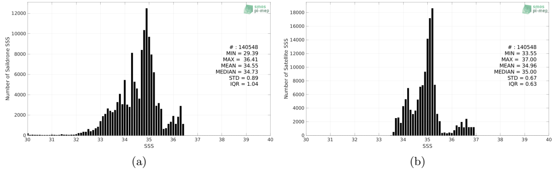
Figure 2: Histograms of SSS from Saildrone (a) and SMOS SSS L4 v2 - Daily (BEC) (b) considering all match-up pairs per bins of 0.1 over the Equatorial Ocean 10N-10S Pi-MEP region and for the full satellite product period.
