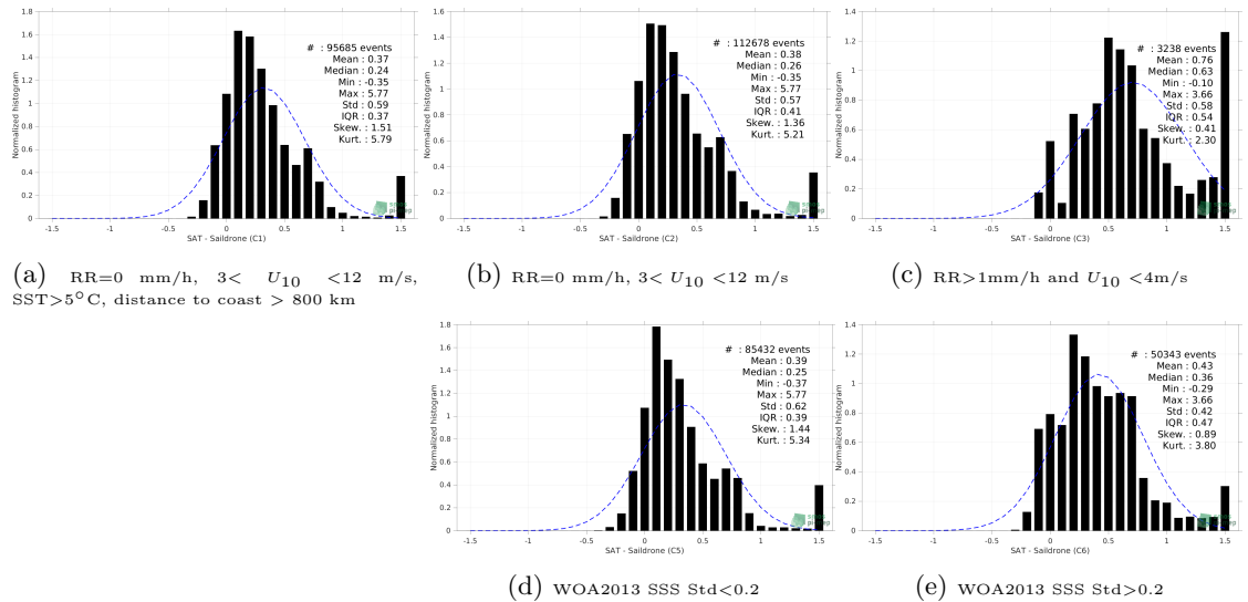
Figure 13: Normalized histogram of \Delta SSS (SMOS SSS L4 v2 - Daily (BEC) - Saldrone) for 5 different subdatasets corresponding to: RR=0 mm/h, 3 < U_{10} < 12 m/s, SST >5^\circ\text{C} , distance to coast > 800 km (a), RR=0 mm/h, 3 < U_{10} < 12 m/s (b), RR >1 mm/h and U_{10} < 4 m/s (c), WOA2013 SSS Std <0.2 (d), WOA2013 SSS Std >0.2 (e).
