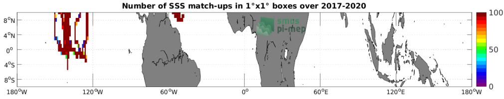
Figure 4: Number of SSS match-ups between Sailldrone SSS and the SMOS SSS L4 v2 - Daily (BEC) SSS product for the Equatorial Ocean 10N-10S Pi-MEP region over 1^\circ \times 1^\circ boxes and for the full satellite product period.
