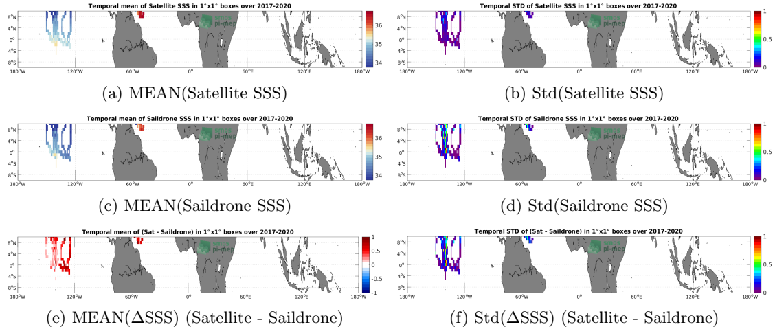
Figure 6: Temporal mean (left) and Std (right) of SSS from SMOS SSS L4 v2 - Daily (BEC) (top), Saildrone (middle), and of \Delta SSS (Satellite - Saildrone). Only match-up pairs are used to generate these maps.
