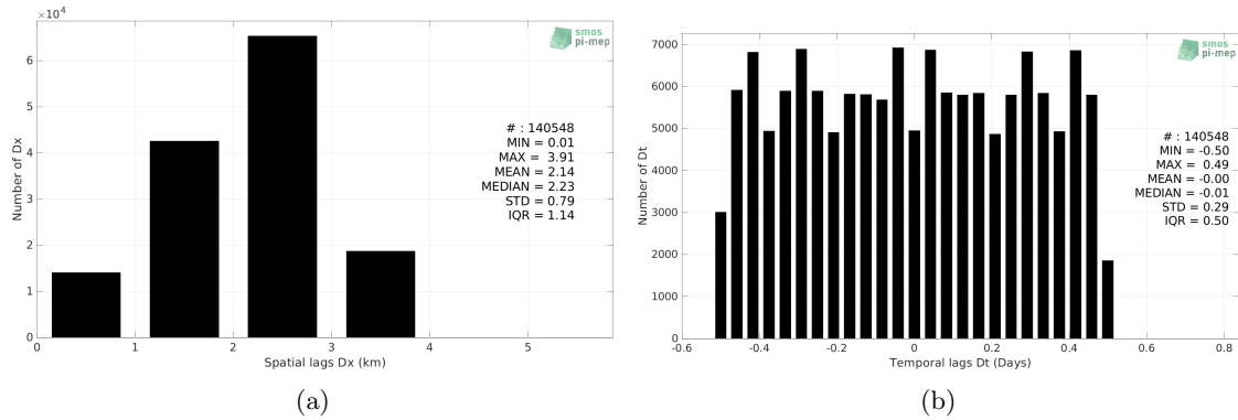
Figure 5: Histograms of the spatial (a) and temporal (b) lags between the location/time of the Sailldrone measurement and the date of the corresponding SMOS SSS L4 v2 - Daily (BEC) SSS pixel.
