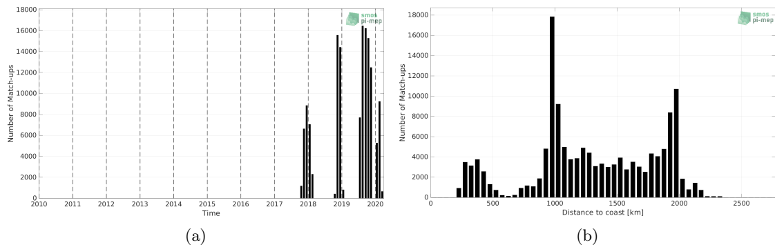
Figure 1: Number of match-ups between Saildrone and SMOS SSS L4 v2 - Daily (BEC) SSS as a function of time (a) and as function of the distance to coast (b) over the Equatorial Ocean 10N-10S Pi-MEP region and for the full satellite product period.
