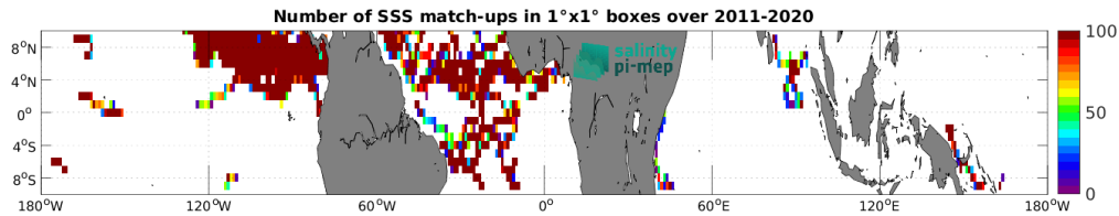
Figure 4: Number of SSS match-ups between Surface drifters SSS and the SMOS SSS L4 v2 - Daily (BEC) SSS product for the Equatorial Ocean 10N-10S Pi-MEP region over 1^\circ \times 1^\circ boxes and for the full satellite product period.
