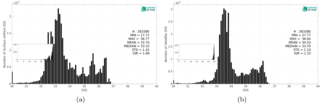
Figure 3: Histograms of SSS from Surface drifters (a) and SMOS SSS L4 v2 - Daily (BEC) (b) considering all match-up pairs per bins of 0.1 over the Equatorial Ocean 10N-10S Pi-MEP region and for the full satellite product period.
