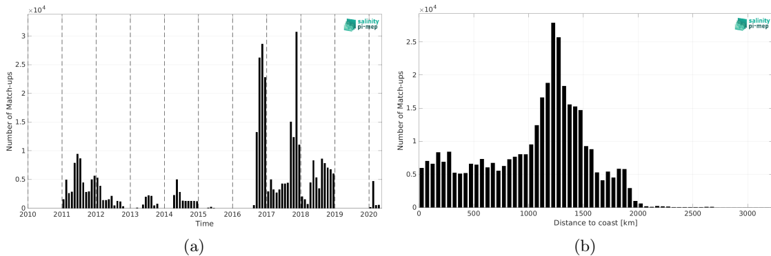
Figure 2: Number of match-ups between Surface drifters and SMOS SSS L4 v2 - Daily (BEC) SSS as a function of time (a) and as function of the distance to coast (b) over the Equatorial Ocean 10N-10S Pi-MEP region and for the full satellite product period.
