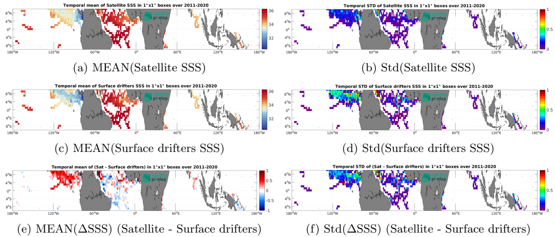
Figure 6: Temporal mean (left) and Std (right) of SSS from SMOS SSS L4 v2 - Daily (BEC) (top), Surface drifters (middle), and of \Delta SSS (Satellite - Surface drifters). Only match-up pairs are used to generate these maps.
