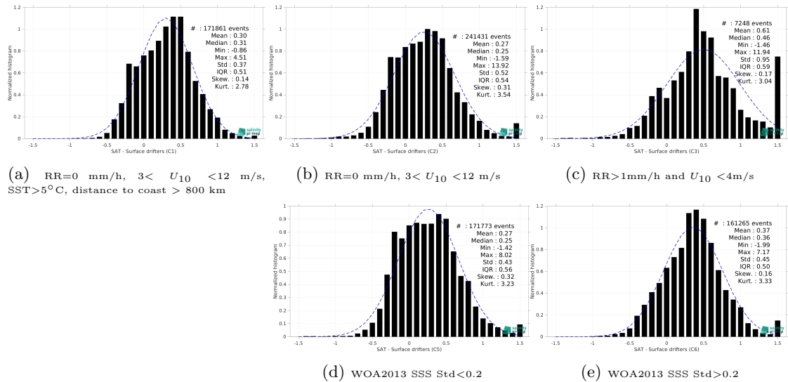
Figure 14: Normalized histogram of \Delta SSS (SMOS SSS L4 v2 - Daily (BEC) - Surface drifters) for 5 different subdatasets corresponding to: RR=0 mm/h, 3 < U_{10} < 12 m/s, SST >5^\circ C, distance to coast > 800 km (a), RR=0 mm/h, 3 < U_{10} < 12 m/s (b), RR >1 mm/h and U_{10} < 4 m/s (c), WOA2013 SSS Std <0.2 (d), WOA2013 SSS Std >0.2 (e).
