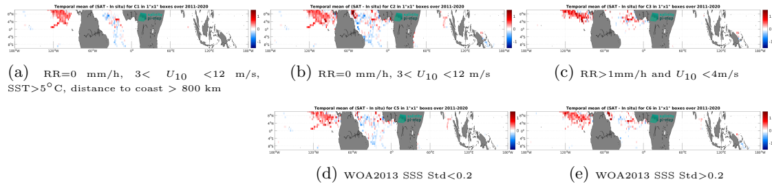
Figure 13: Temporal mean gridded over spatial boxes of size 1^\circ \times 1^\circ of \Delta SSS (SMOS SSS L4 v2 - Daily (BEC) - Surface drifters) for 5 different subdatasets corresponding to:RR=0 mm/h, 3 < U_{10} < 12 m/s, SST >5^\circ C, distance to coast > 800 km (a), RR=0 mm/h, 3 < U_{10} < 12 m/s (b), RR >1 mm/h and U_{10} < 4 m/s (c), WOA2013 SSS Std <0.2 (d), WOA2013 SSS Std >0.2 (e).
