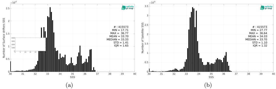
Figure 2: Histograms of SSS from Surface drifters (a) and SMOS SSS L4 v2 - Daily (BEC) (b) considering all match-up pairs per bins of 0.1 over the Equatorial Ocean 10N-10S Pi-MEP region and for the full satellite product period.
