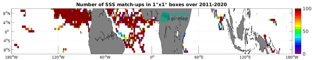
Figure 3: Number of SSS match-ups between Surface drifters SSS and the SMOS SSS L4 v2 - Daily (BEC) SSS product for the Equatorial Ocean 10N-10S Pi-MEP region over 1^\circ \times 1^\circ boxes and for the full satellite product period.
