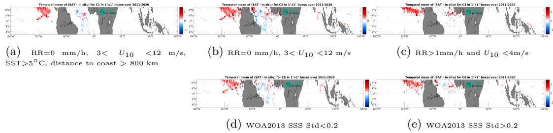
Figure 11: Temporal mean gridded over spatial boxes of size 1^\circ \times 1^\circ of \Delta SSS (SMOS SSS L4 v2 - Daily (BEC) - Surface drifters) for 5 different subdatasets corresponding to:RR=0 mm/h, 3 < U_{10} < 12 m/s, SST >5^\circ C, distance to coast > 800 km (a), RR=0 mm/h, 3 < U_{10} < 12 m/s (b), RR >1 mm/h and U_{10} < 4 m/s (c), WOA2013 SSS Std <0.2 (d), WOA2013 SSS Std >0.2 (e).
