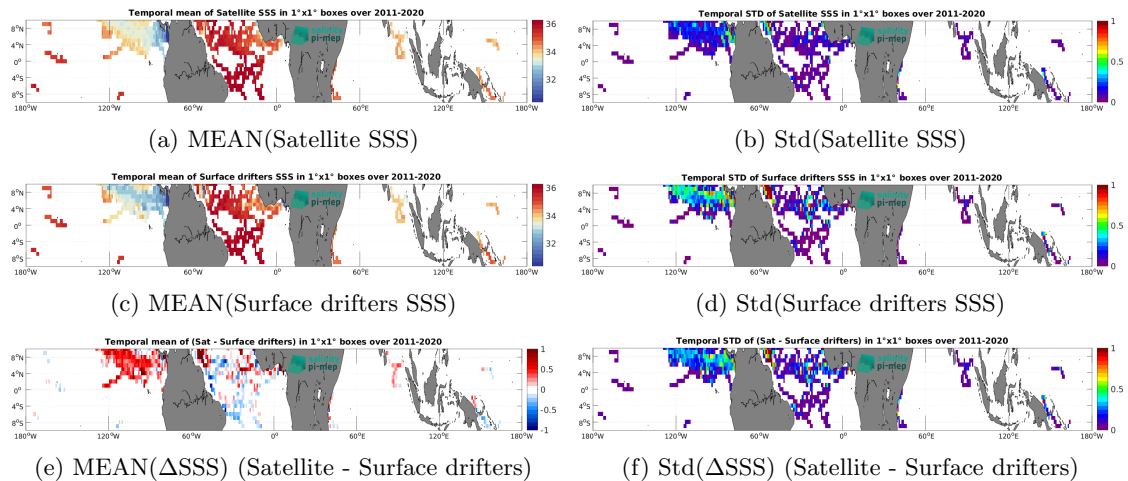
Figure 5: Temporal mean (left) and Std (right) of SSS from SMOS SSS L4 v2 - Daily (BEC) (top), Surface drifters (middle), and of \Delta SSS (Satellite - Surface drifters). Only match-up pairs are used to generate these maps.
