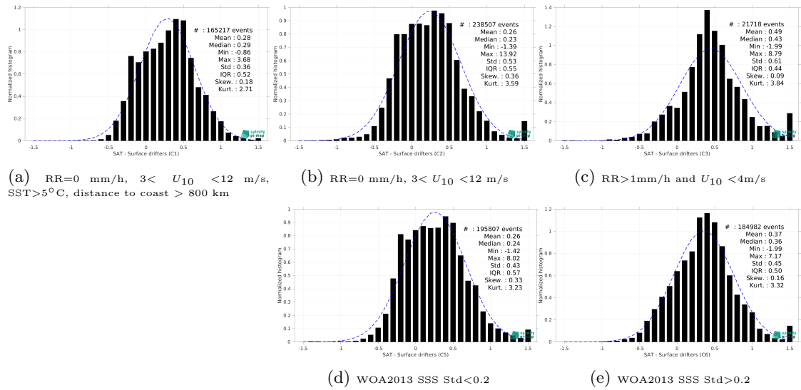
Figure 12: Normalized histogram of \Delta SSS (SMOS SSS L4 v2 - Daily (BEC) - Surface drifters) for 5 different subdatasets corresponding to: RR=0 mm/h, 3 < U_{10} < 12 m/s, SST >5^\circ C, distance to coast > 800 km (a), RR=0 mm/h, 3 < U_{10} < 12 m/s (b), RR >1 mm/h and U_{10} < 4 m/s (c), WOA2013 SSS Std <0.2 (d), WOA2013 SSS Std >0.2 (e).
