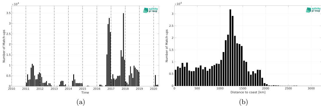
Figure 1: Number of match-ups between Surface drifters and SMOS SSS L4 v2 - Daily (BEC) SSS as a function of time (a) and as function of the distance to coast (b) over the Equatorial Ocean 10N-10S Pi-MEP region and for the full satellite product period.
