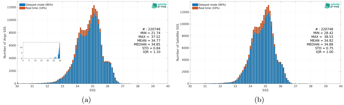
Figure 2: Histograms of SSS from Argo (a) and SMOS SSS L4 v2 - Daily (BEC) (b) considering all match-up pairs per bins of 0.1 over the Equatorial Ocean 10N-10S Pi-MEP region and for the full satellite product period.
