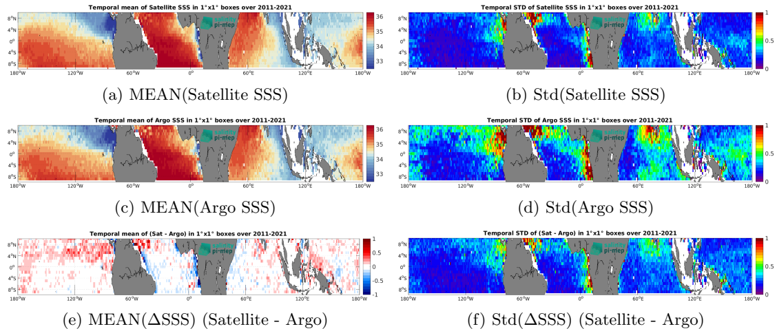
Figure 6: Temporal mean (left) and Std (right) of SSS from SMOS SSS L4 v2 - Daily (BEC) (top), Argo (middle), and of \Delta SSS (Satellite - Argo). Only match-up pairs are used to generate these maps.
