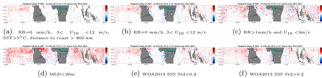
Figure 12: Temporal mean gridded over spatial boxes of size 1^\circ \times 1^\circ of \Delta SSS (SMOS SSS L4 v2 - Daily (BEC) - Argo) for 6 different subdatasets corresponding to:RR=0 mm/h, 3 < U_{10} < 12 m/s, SST >5^\circ C, distance to coast > 800 km (a), RR=0 mm/h, 3 < U_{10} < 12 m/s (b), RR >1 mm/h and U_{10} < 4 m/s (c),MLD <20 m (d),WOA2013 SSS Std <0.2 (e),WOA2013 SSS Std >0.2 (f).
