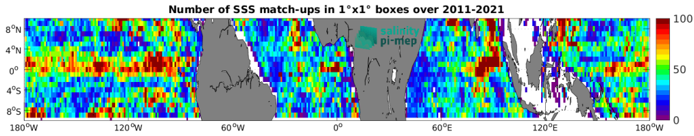
Figure 4: Number of SSS match-ups between Argo SSS and the SMOS SSS L4 v2 - Daily (BEC) SSS product for the Equatorial Ocean 10N-10S Pi-MEP region over 1^\circ \times 1^\circ boxes and for the full satellite product period.
