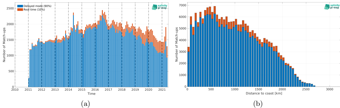
Figure 1: Number of match-ups between Argo and SMOS SSS L4 v2 - Daily (BEC) SSS as a function of time (a) and as function of the distance to coast (b) over the Equatorial Ocean 10N-10S Pi-MEP region and for the full satellite product period.
