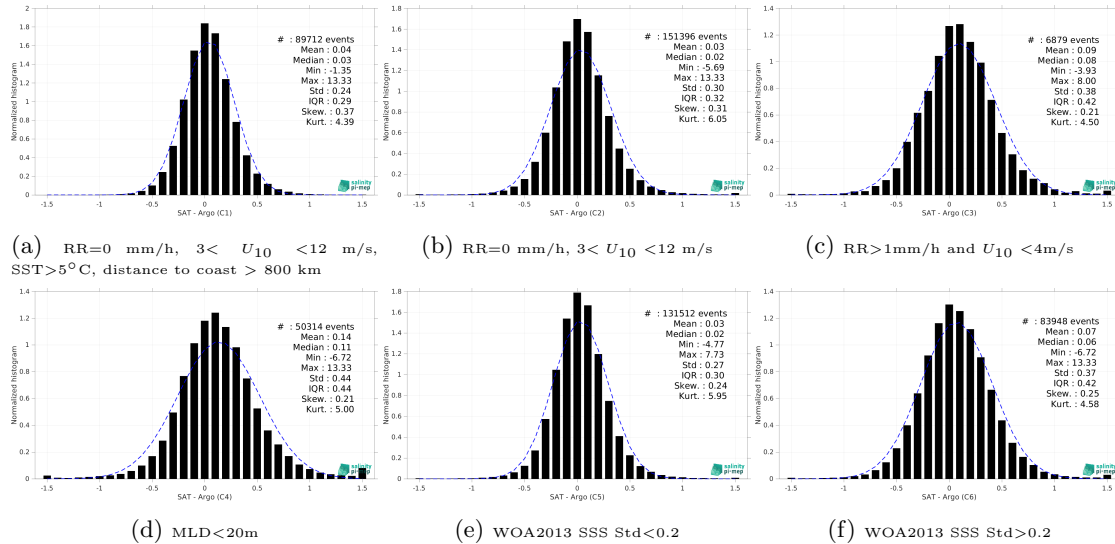
Figure 13: Normalized histogram of \Delta SSS (SMOS SSS L4 v2 - Daily (BEC) - Argo) for 6 different subdatasets corresponding to: RR=0 mm/h, 3 < U_{10} < 12 m/s, SST >5^\circ C, distance to coast > 800 km (a), RR=0 mm/h, 3 < U_{10} < 12 m/s (b), RR >1 mm/h and U_{10} < 4 m/s (c), MLD <20 m (d), WOA2013 SSS Std <0.2 (e), WOA2013 SSS Std >0.2 (f).
