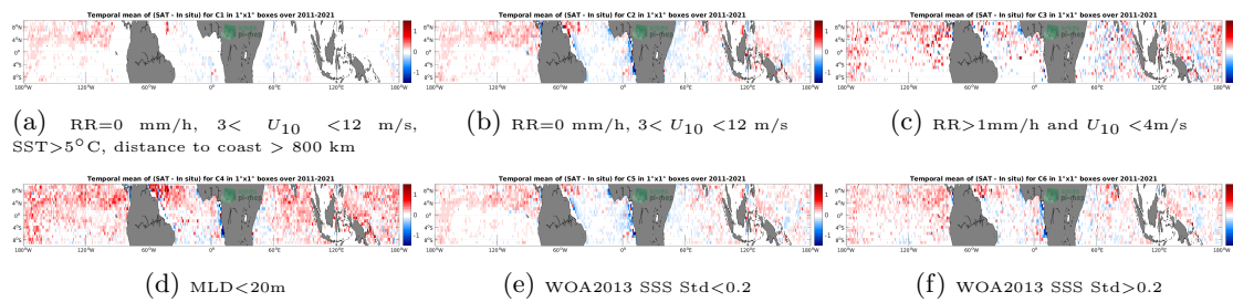
Figure 12: Temporal mean gridded over spatial boxes of size 1^\circ \times 1^\circ of \Delta\text{SSS} (SMOS SSS L4 v2 - Daily (BEC) - Argo) for 6 different subdatasets corresponding to:RR=0 mm/h, 3 < U_{10} < 12 m/s, SST>5°C, distance to coast > 800 km (a), RR=0 mm/h, 3 < U_{10} < 12 m/s (b), RR>1mm/h and U_{10} < 4 m/s (c),MLD<20m (d),WOA2013 SSS Std<0.2 (e),WOA2013 SSS Std>0.2 (f).
