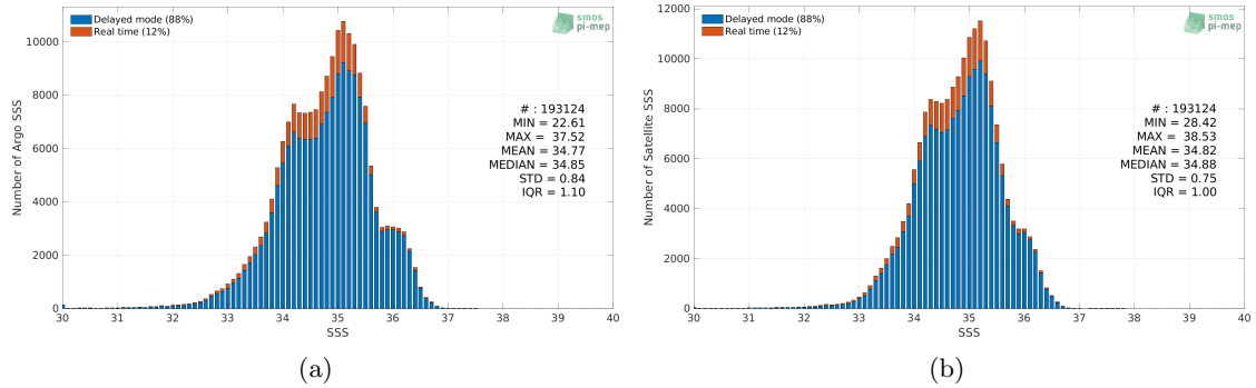
Figure 2: Histograms of SSS from Argo (a) and SMOS SSS L4 v2 - Daily (BEC) (b) considering all match-up pairs per bins of 0.1 over the Equatorial Ocean 10N-10S Pi-MEP region and for the full satellite product period.
