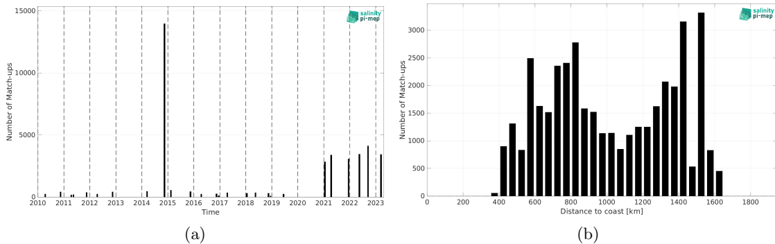
Figure 2: Number of match-ups between TSG (Polarstern) and SMOS SSS L2Q v331 - With FLAG (CMEMS-CATDS-CPDC) SSS as a function of time (a) and as function of the distance to coast (b) over the Equatorial Ocean 10N-10S Pi-MEP region and for the full satellite product period.
