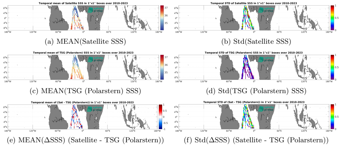
Figure 7: Temporal mean (left) and Std (right) of SSS from SMOS SSS L2Q v331 - With FLAG (CMEMS-CATDS-CPDC) (top), TSG (Polarstern) (middle), and of \Delta SSS (Satellite - TSG (Polarstern)). Only match-up pairs are used to generate these maps.
