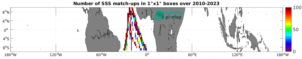
Figure 5: Number of SSS match-ups between TSG (Polarstern) SSS and the SMOS SSS L2Q v331 - With FLAG (CMEMS-CATDS-CPDC) SSS product for the Equatorial Ocean 10N-10S Pi-MEP region over 1^\circ \times 1^\circ boxes and for the full satellite product period.
