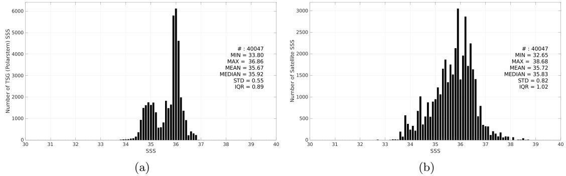
Figure 3: Histograms of SSS from TSG (Polarstern) (a) and SMOS SSS L2Q v331 - With FLAG (CMEMS-CATDS-CPDC) (b) considering all match-up pairs per bins of 0.1 over the Equatorial Ocean 10N-10S Pi-MEP region and for the full satellite product period.
