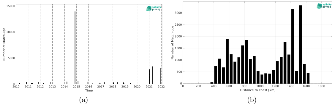
Figure 1: Number of match-ups between TSG (Polarstern) and SMOS SSS L2Q v331 - With FLAG (CMEMS-CATDS-CPDC) SSS as a function of time (a) and as function of the distance to coast (b) over the Equatorial Ocean 10N-10S Pi-MEP region and for the full satellite product period.
