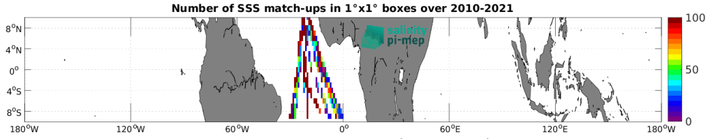
Figure 4: Number of SSS match-ups between TSG (Polarstern) SSS and the SMOS SSS L2Q v331 - With FLAG (CMEMS-CATDS-CPDC) SSS product for the Equatorial Ocean 10N-10S Pi-MEP region over 1^\circ \times 1^\circ boxes and for the full satellite product period.
