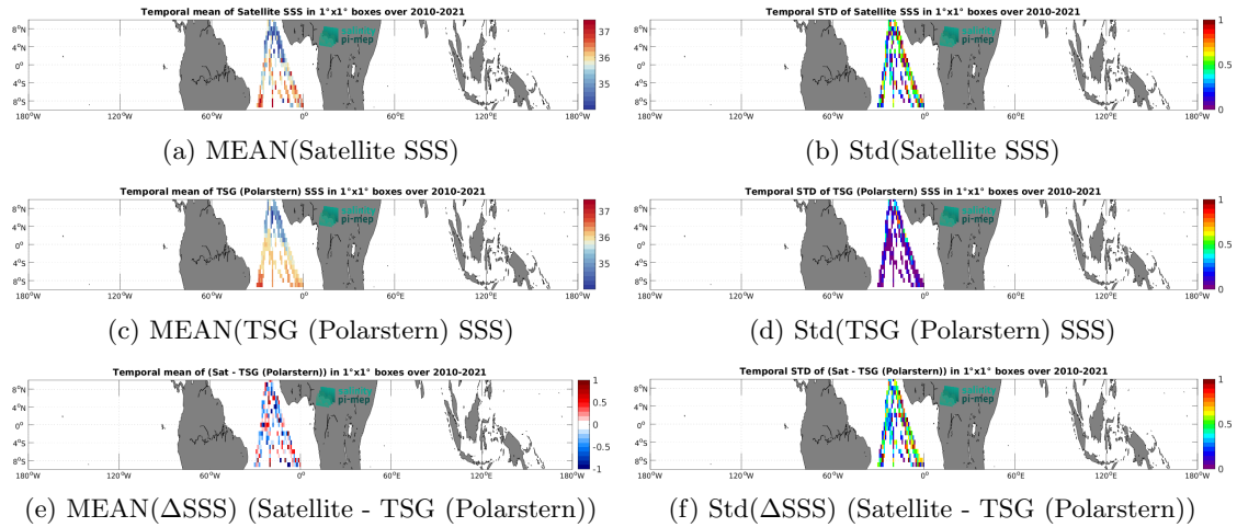
Figure 6: Temporal mean (left) and Std (right) of SSS from SMOS SSS L2Q v331 - With FLAG (CMEMS-CATDS-CPDC) (top), TSG (Polarstern) (middle), and of \Delta SSS (Satellite - TSG (Polarstern)). Only match-up pairs are used to generate these maps.
