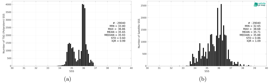
Figure 2: Histograms of SSS from TSG (Polarstern) (a) and SMOS SSS L2Q v331 - With FLAG (CMEMS-CATDS-CPDC) (b) considering all match-up pairs per bins of 0.1 over the Equatorial Ocean 10N-10S Pi-MEP region and for the full satellite product period.
