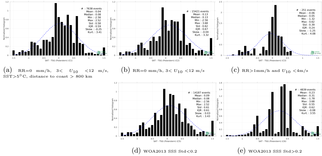
Figure 13: Normalized histogram of \Delta\text{SSS} (SMOS SSS L2Q v331 - With FLAG (CMEMS-CATDS-CPDC) - TSG (Polarstern)) for 5 different subdatasets corresponding to: RR=0 mm/h, 3 < U_{10} < 12 m/s, SST>5°C, distance to coast > 800 km (a), RR=0 mm/h, 3 < U_{10} < 12 m/s (b), RR>1mm/h and U_{10} < 4 m/s (c), WOA2013 SSS Std<0.2 (d), WOA2013 SSS Std>0.2 (e).
