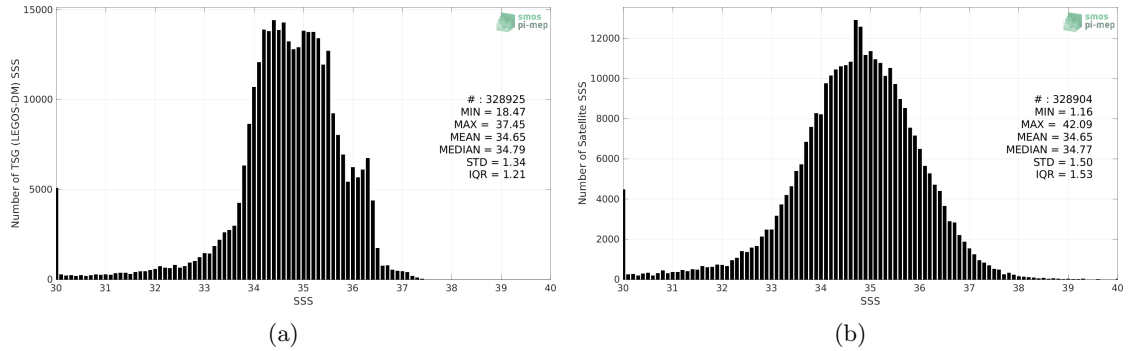
Figure 2: Histograms of SSS from TSG (LEGOS-DM) (a) and SMOS SSS L2Q v331 - With FLAG (CMEMS-CATDS-CPDC) (b) considering all match-up pairs per bins of 0.1 over the Equatorial Ocean 10N-10S Pi-MEP region and for the full satellite product period.
