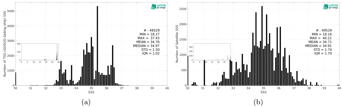
Figure 3: Histograms of SSS from TSG (GOSUD-Sailing-ship) (a) and SMOS SSS L2Q v331 - With FLAG (CMEMS-CATDS-CPDC) (b) considering all match-up pairs per bins of 0.1 over the Equatorial Ocean 10N-10S Pi-MEP region and for the full satellite product period.
