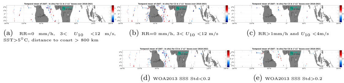
Figure 14: Temporal mean gridded over spatial boxes of size 1^\circ \times 1^\circ of \Delta SSS (SMOS SSS L2Q v331 - With FLAG (CMEMS-CATDS-CPDC) - TSG (GOSUD-Sailing-ship)) for 5 different subdatasets corresponding to:RR=0 mm/h, 3 < U_{10} < 12 m/s, SST >5^\circ C, distance to coast > 800 km (a), RR=0 mm/h, 3 < U_{10} < 12 m/s (b), RR >1 mm/h and U_{10} < 4 m/s (c), WOA2013 SSS Std <0.2 (d), WOA2013 SSS Std >0.2 (e).
