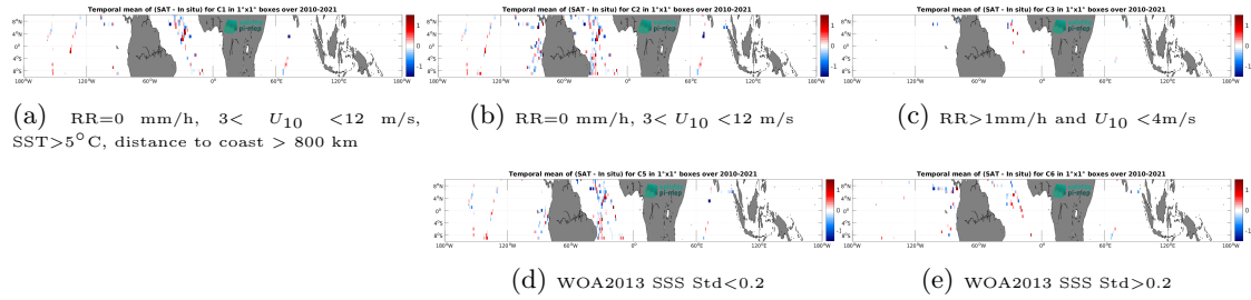
Figure 12: Temporal mean gridded over spatial boxes of size 1^{\circ}\times 1^{\circ} of \Delta SSS (SMOS SSS L2Q v331 - With FLAG (CMEMS-CATDS-CPDC) - TSG (GOSUD-Sailing-ship)) for 5 different subdatasets corresponding to: RR=0 mm/h, 3 < U_{10} < 12 m/s, SST > 5^{\circ}\text{C} , distance to coast > 800 km (a), RR=0 mm/h, 3 < U_{10} < 12 m/s (b), RR > 1 mm/h and U_{10} < 4 m/s (c), WOA2013 SSS Std < 0.2 (d), WOA2013 SSS Std > 0.2 (e).
