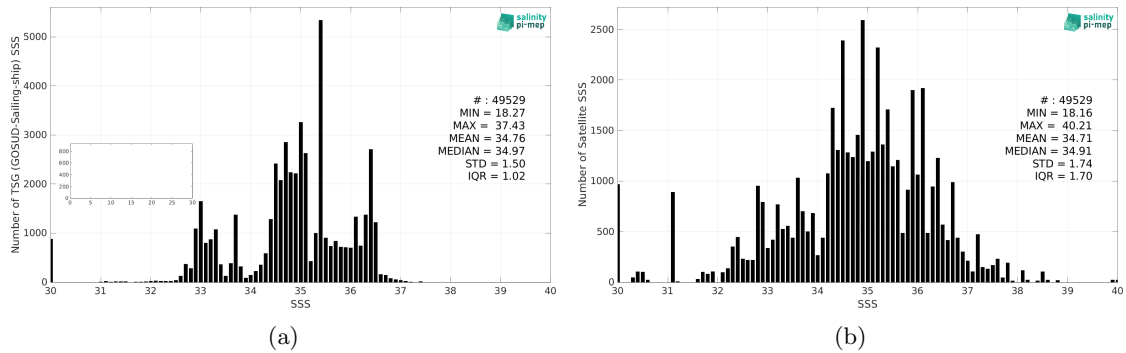
Figure 2: Histograms of SSS from TSG (GOSUD-Sailing-ship) (a) and SMOS SSS L2Q v331 - With FLAG (CMEMS-CATDS-CPDC) (b) considering all match-up pairs per bins of 0.1 over the Equatorial Ocean 10N-10S Pi-MEP region and for the full satellite product period.
