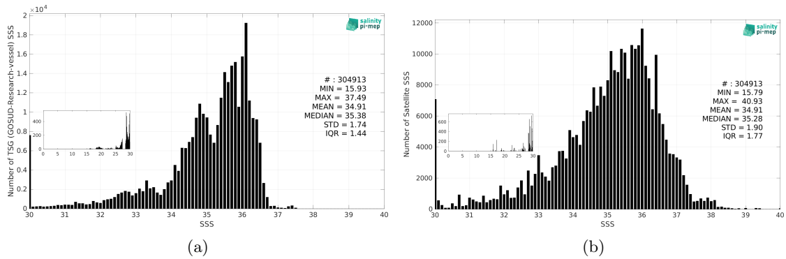
Figure 3: Histograms of SSS from TSG (GOSUD-Research-vessel) (a) and SMOS SSS L2Q v331 - With FLAG (CMEMS-CATDS-CPDC) (b) considering all match-up pairs per bins of 0.1 over the Equatorial Ocean 10N-10S Pi-MEP region and for the full satellite product period.
