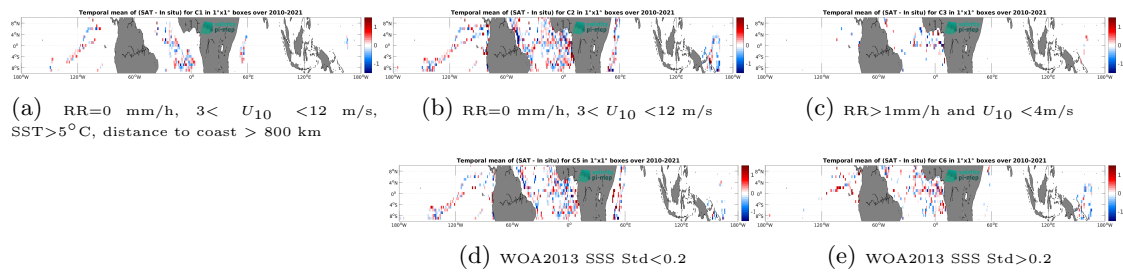
Figure 14: Temporal mean gridded over spatial boxes of size 1^\circ \times 1^\circ of \Delta SSS (SMOS SSS L2Q v331 - With FLAG (CMEMS-CATDS-CPDC) - TSG (GOSUD-Research-vessel)) for 5 different subdatasets corresponding to:RR=0 mm/h, 3 < U_{10} < 12 m/s, SST >5^\circ\text{C} , distance to coast > 800 km (a), RR=0 mm/h, 3 < U_{10} < 12 m/s (b), RR >1 mm/h and U_{10} < 4 m/s (c), WOA2013 SSS Std <0.2 (d), WOA2013 SSS Std >0.2 (e).
