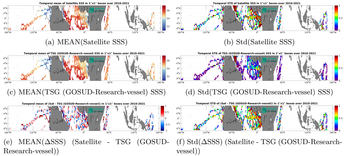
Figure 7: Temporal mean (left) and Std (right) of SSS from SMOS SSS L2Q v331 - With FLAG (CMEMS-CATDS-CPDC) (top), TSG (GOSUD-Research-vessel) (middle), and of \Delta SSS (Satellite - TSG (GOSUD-Research-vessel)). Only match-up pairs are used to generate these maps.
