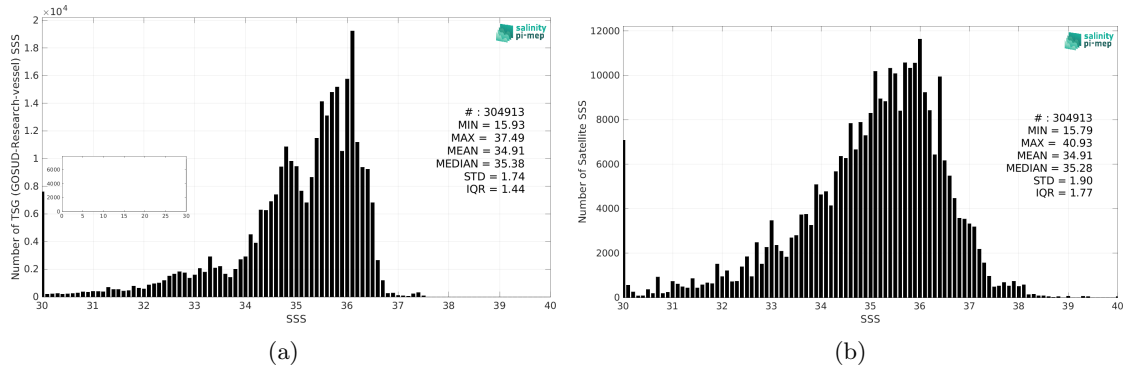
Figure 2: Histograms of SSS from TSG (GOSUD-Research-vessel) (a) and SMOS SSS L2Q v331 - With FLAG (CMEMS-CATDS-CPDC) (b) considering all match-up pairs per bins of 0.1 over the Equatorial Ocean 10N-10S Pi-MEP region and for the full satellite product period.
