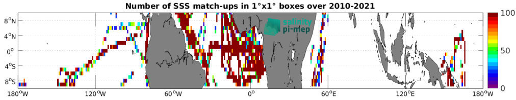
Figure 4: Number of SSS match-ups between TSG (GOSUD-Research-vessel) SSS and the SMOS SSS L2Q v331 - With FLAG (CMEMS-CATDS-CPDC) SSS product for the Equatorial Ocean 10N-10S Pi-MEP region over 1^\circ \times 1^\circ boxes and for the full satellite product period.
