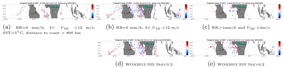
Figure 12: Temporal mean gridded over spatial boxes of size 1^\circ \times 1^\circ of \Delta SSS (SMOS SSS L2Q v331 - With FLAG (CMEMS-CATDS-CPDC) - TSG (GOSUD-Research-vessel)) for 5 different subdatasets corresponding to:RR=0 mm/h, 3 < U_{10} < 12 m/s, SST >5^\circ C, distance to coast > 800 km (a), RR=0 mm/h, 3 < U_{10} < 12 m/s (b), RR >1 mm/h and U_{10} < 4 m/s (c), WOA2013 SSS Std <0.2 (d), WOA2013 SSS Std >0.2 (e).
