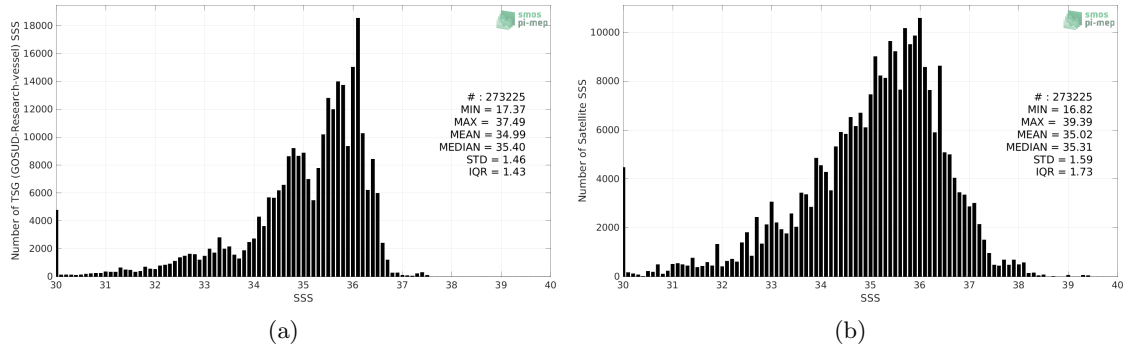
Figure 2: Histograms of SSS from TSG (GOSUD-Research-vessel) (a) and SMOS SSS L2Q v331 - With FLAG (CMEMS-CATDS-CPDC) (b) considering all match-up pairs per bins of 0.1 over the Equatorial Ocean 10N-10S Pi-MEP region and for the full satellite product period.
