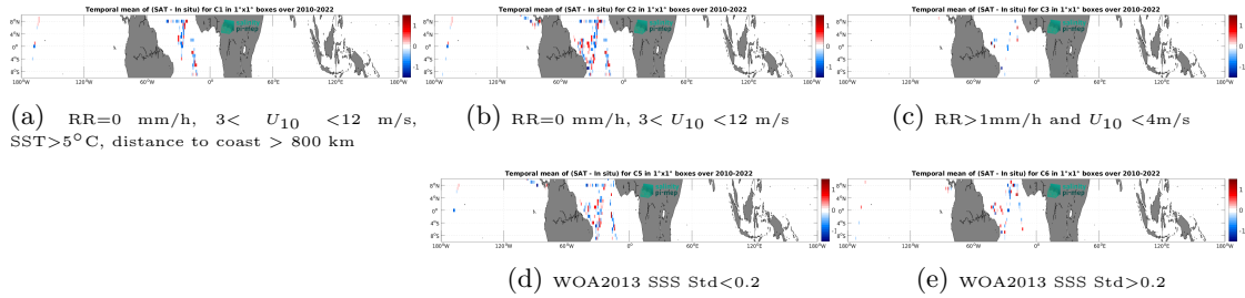
Figure 14: Temporal mean gridded over spatial boxes of size 1^\circ \times 1^\circ of \Delta SSS (SMOS SSS L2Q v331 - With FLAG (CMEMS-CATDS-CPDC) - TSG (CSIC-UTM)) for 5 different subdatasets corresponding to: RR=0 mm/h, 3 < U_{10} < 12 m/s, SST>5°C, distance to coast > 800 km (a), RR=0 mm/h, 3 < U_{10} < 12 m/s (b), RR>1mm/h and U_{10} < 4 m/s (c), WOA2013 SSS Std<0.2 (d), WOA2013 SSS Std>0.2 (e).
