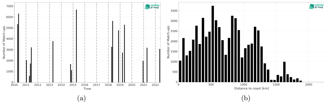
Figure 2: Number of match-ups between TSG (CSIC-UTM) and SMOS SSS L2Q v331 - With FLAG (CMEMS-CATDS-CPDC) SSS as a function of time (a) and as function of the distance to coast (b) over the Equatorial Ocean 10N-10S Pi-MEP region and for the full satellite product period.
