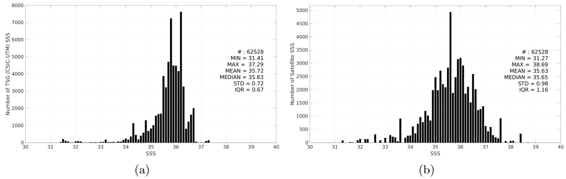
Figure 3: Histograms of SSS from TSG (CSIC-UTM) (a) and SMOS SSS L2Q v331 - With FLAG (CMEMS-CATDS-CPDC) (b) considering all match-up pairs per bins of 0.1 over the Equatorial Ocean 10N-10S Pi-MEP region and for the full satellite product period.
