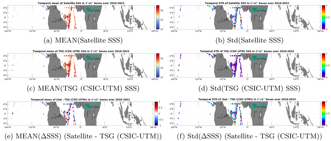
Figure 7: Temporal mean (left) and Std (right) of SSS from SMOS SSS L2Q v331 - With FLAG (CMEMS-CATDS-CPDC) (top), TSG (CSIC-UTM) (middle), and of \Delta SSS (Satellite - TSG (CSIC-UTM)). Only match-up pairs are used to generate these maps.
