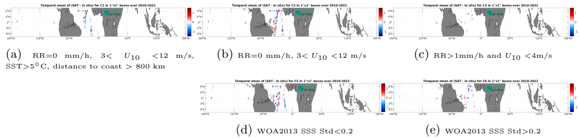
Figure 12: Temporal mean gridded over spatial boxes of size 1^{\circ}\times 1^{\circ} of \Delta\text{SSS} (SMOS SSS L2Q v331 - With FLAG (CMEMS-CATDS-CPDC) - TSG (CSIC-UTM)) for 5 different subdatasets corresponding to:RR=0 mm/h, 3 < U_{10} < 12 m/s, SST >5^{\circ}\text{C} , distance to coast > 800 km (a), RR=0 mm/h, 3 < U_{10} < 12 m/s (b), RR >1 mm/h and U_{10} < 4 m/s (c), WOA2013 SSS Std <0.2 (d), WOA2013 SSS Std >0.2 (e).
