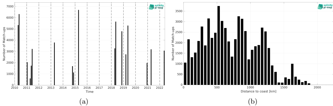
Figure 1: Number of match-ups between TSG (CSIC-UTM) and SMOS SSS L2Q v331 - With FLAG (CMEMS-CATDS-CPDC) SSS as a function of time (a) and as function of the distance to coast (b) over the Equatorial Ocean 10N-10S Pi-MEP region and for the full satellite product period.
