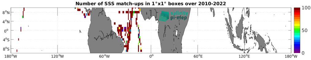
Figure 4: Number of SSS match-ups between TSG (CSIC-UTM) SSS and the SMOS SSS L2Q v331 - With FLAG (CMEMS-CATDS-CPDC) SSS product for the Equatorial Ocean 10N-10S Pi-MEP region over 1^\circ \times 1^\circ boxes and for the full satellite product period.
