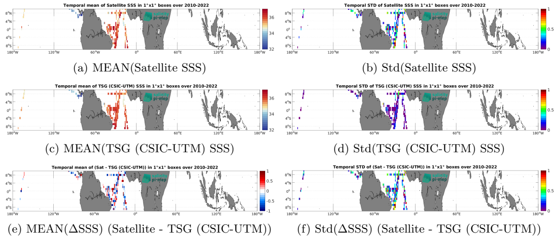
Figure 6: Temporal mean (left) and Std (right) of SSS from SMOS SSS L2Q v331 - With FLAG (CMEMS-CATDS-CPDC) (top), TSG (CSIC-UTM) (middle), and of \Delta SSS (Satellite - TSG (CSIC-UTM)). Only match-up pairs are used to generate these maps.
