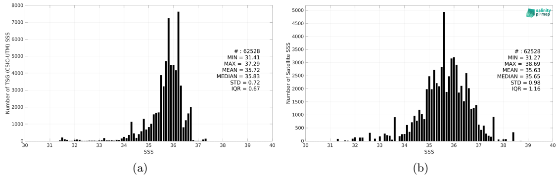
Figure 2: Histograms of SSS from TSG (CSIC-UTM) (a) and SMOS SSS L2Q v331 - With FLAG (CMEMS-CATDS-CPDC) (b) considering all match-up pairs per bins of 0.1 over the Equatorial Ocean 10N-10S Pi-MEP region and for the full satellite product period.
