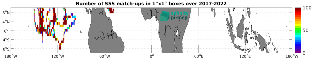
Figure 5: Number of SSS match-ups between Saildrone SSS and the SMOS SSS L2Q v331 - With FLAG (CMEMS-CATDS-CPDC) SSS product for the Equatorial Ocean 10N-10S Pi-MEP region over 1^\circ \times 1^\circ boxes and for the full satellite product period.
