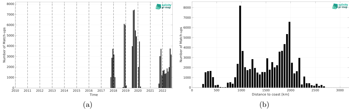
Figure 2: Number of match-ups between Saildrone and SMOS SSS L2Q v331 - With FLAG (CMEMS-CATDS-CPDC) SSS as a function of time (a) and as function of the distance to coast (b) over the Equatorial Ocean 10N-10S Pi-MEP region and for the full satellite product period.
