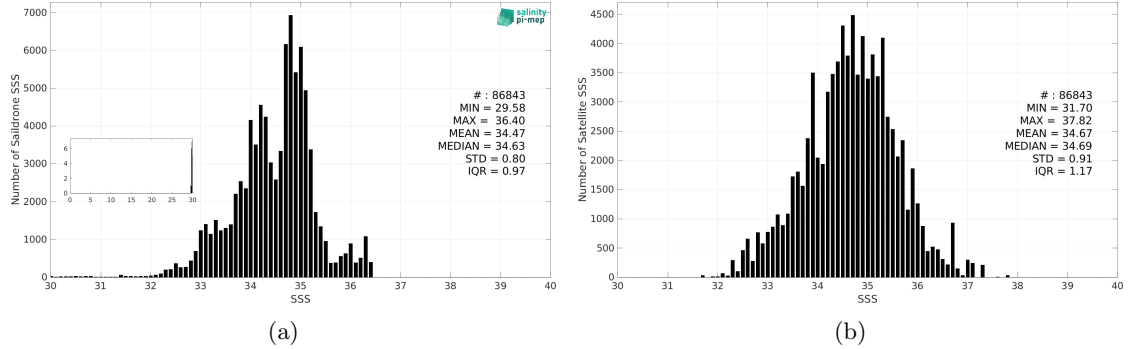
Figure 3: Histograms of SSS from Saildrone (a) and SMOS SSS L2Q v331 - With FLAG (CMEMS-CATDS-CPDC) (b) considering all match-up pairs per bins of 0.1 over the Equatorial Ocean 10N-10S Pi-MEP region and for the full satellite product period.
