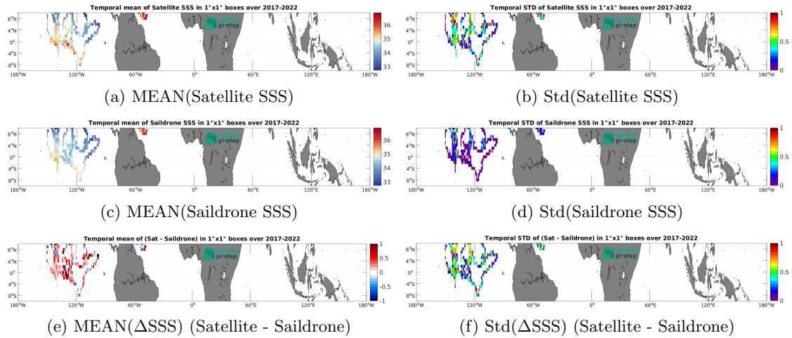
Figure 7: Temporal mean (left) and Std (right) of SSS from SMOS SSS L2Q v331 - With FLAG (CMEMS-CATDS-CPDC) (top), Saildrone (middle), and of \Delta SSS (Satellite - Saildrone). Only match-up pairs are used to generate these maps.
