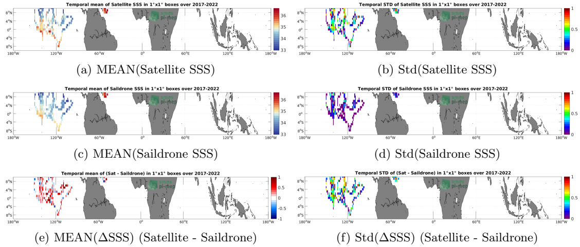
Figure 6: Temporal mean (left) and Std (right) of SSS from SMOS SSS L2Q v331 - With FLAG (CMEMS-CATDS-CPDC) (top), Saildrone (middle), and of \Delta SSS (Satellite - Saildrone). Only match-up pairs are used to generate these maps.
