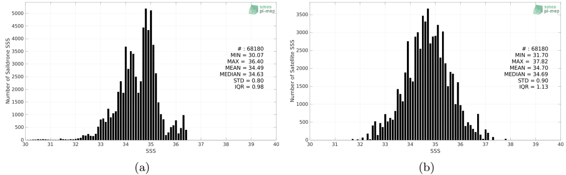
Figure 2: Histograms of SSS from Saildrone (a) and SMOS SSS L2Q v331 - With FLAG (CMEMS-CATDS-CPDC) (b) considering all match-up pairs per bins of 0.1 over the Equatorial Ocean 10N-10S Pi-MEP region and for the full satellite product period.
