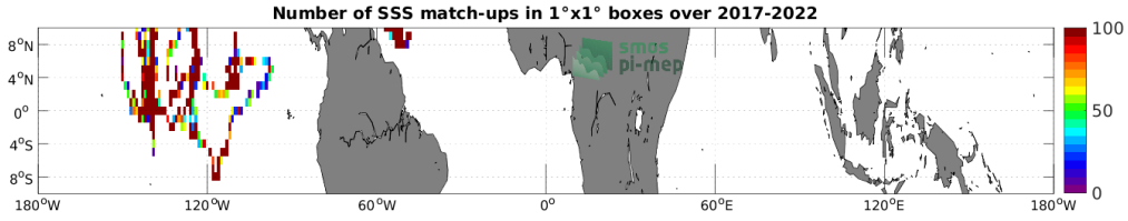
Figure 4: Number of SSS match-ups between Saildrone SSS and the SMOS SSS L2Q v331 - With FLAG (CMEMS-CATDS-CPDC) SSS product for the Equatorial Ocean 10N-10S Pi-MEP region over 1^\circ \times 1^\circ boxes and for the full satellite product period.
