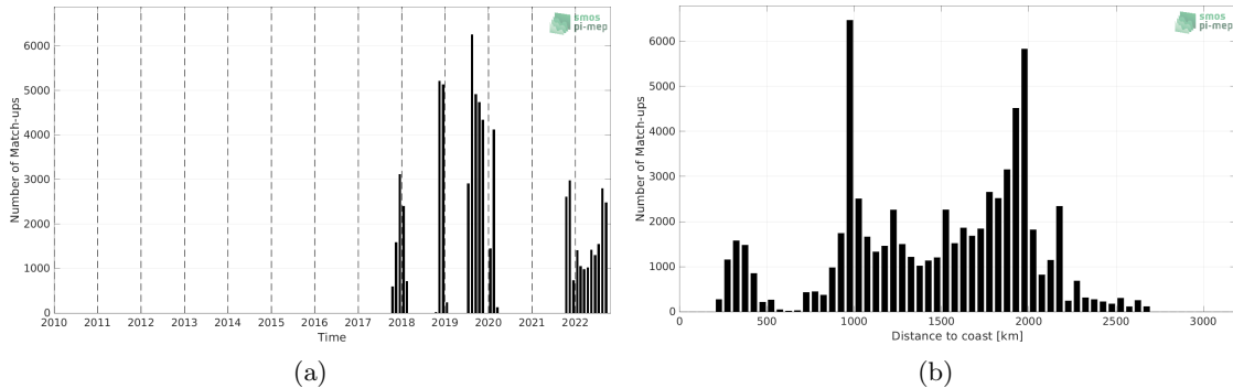
Figure 1: Number of match-ups between Saildrone and SMOS SSS L2Q v331 - With FLAG (CMEMS-CATDS-CPDC) SSS as a function of time (a) and as function of the distance to coast (b) over the Equatorial Ocean 10N-10S Pi-MEP region and for the full satellite product period.
