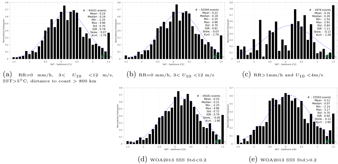
Figure 13: Normalized histogram of \Delta SSS (SMOS SSS L2Q v331 - With FLAG (CMEMS-CATDS-CPDC) - Saildrone) for 5 different subdatasets corresponding to: RR=0 mm/h, 3 < U_{10} < 12 m/s, SST > 5^\circ C , distance to coast > 800 km (a), RR=0 mm/h, 3 < U_{10} < 12 m/s (b), RR >1 mm/h and U_{10} < 4 m/s (c), WOA2013 SSS Std <0.2 (d), WOA2013 SSS Std >0.2 (e).
