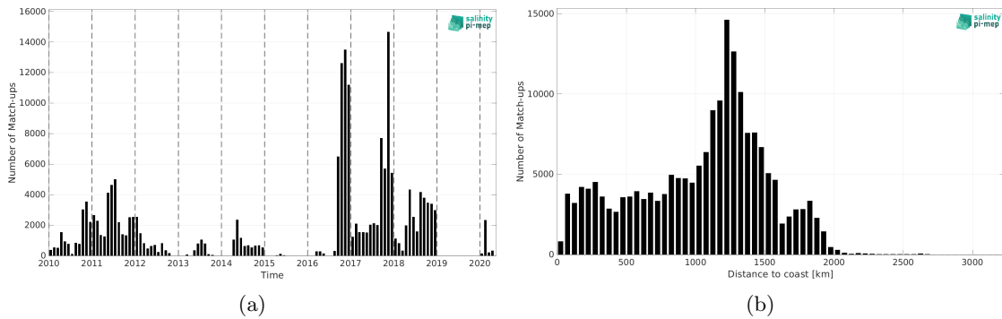
Figure 1: Number of match-ups between Surface drifters and SMOS SSS L2Q v331 - With FLAG (CMEMS-CATDS-CPDC) SSS as a function of time (a) and as function of the distance to coast (b) over the Equatorial Ocean 10N-10S Pi-MEP region and for the full satellite product period.
