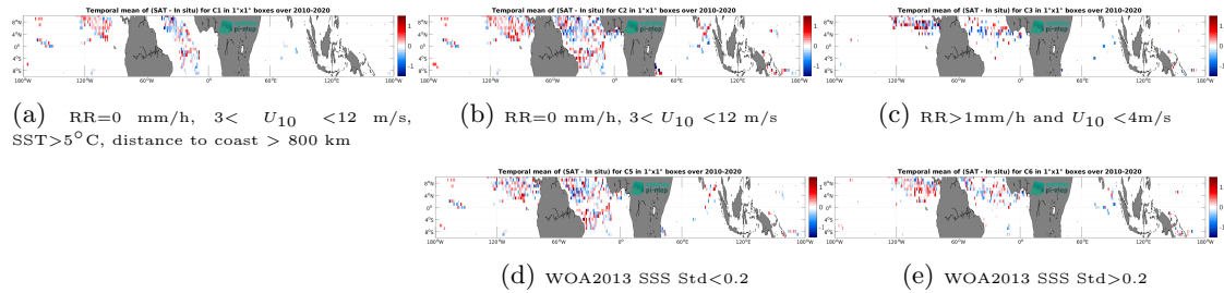
Figure 11: Temporal mean gridded over spatial boxes of size 1^\circ \times 1^\circ of \Delta SSS (SMOS SSS L2Q v331 - With FLAG (CMEMS-CATDS-CPDC) - Surface drifters) for 5 different subdatasets corresponding to:RR=0 mm/h, 3 < U_{10} < 12 m/s, SST >5^\circ C, distance to coast > 800 km (a), RR=0 mm/h, 3 < U_{10} < 12 m/s (b), RR >1 mm/h and U_{10} < 4 m/s (c), WOA2013 SSS Std <0.2 (d), WOA2013 SSS Std >0.2 (e).
