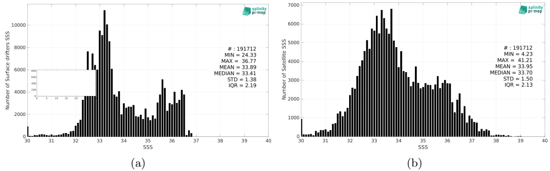
Figure 2: Histograms of SSS from Surface drifters (a) and SMOS SSS L2Q v331 - With FLAG (CMEMS-CATDS-CPDC) (b) considering all match-up pairs per bins of 0.1 over the Equatorial Ocean 10N-10S Pi-MEP region and for the full satellite product period.
