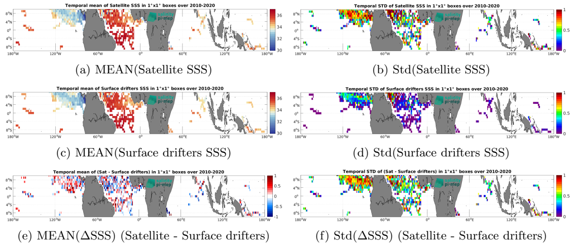
Figure 5: Temporal mean (left) and Std (right) of SSS from SMOS SSS L2Q v331 - With FLAG (CMEMS-CATDS-CPDC) (top), Surface drifters (middle), and of \Delta SSS (Satellite - Surface drifters). Only match-up pairs are used to generate these maps.
