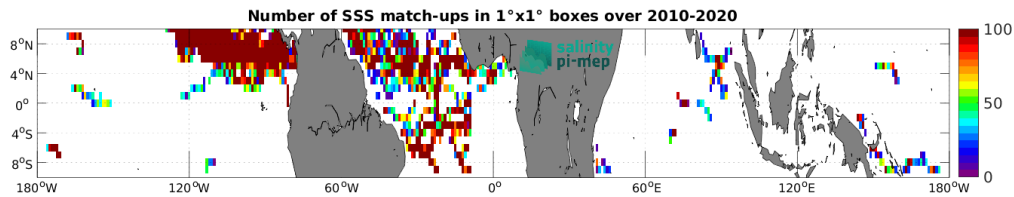
Figure 3: Number of SSS match-ups between Surface drifters SSS and the SMOS SSS L2Q v331 - With FLAG (CMEMS-CATDS-CPDC) SSS product for the Equatorial Ocean 10N-10S Pi-MEP region over 1^\circ \times 1^\circ boxes and for the full satellite product period.
