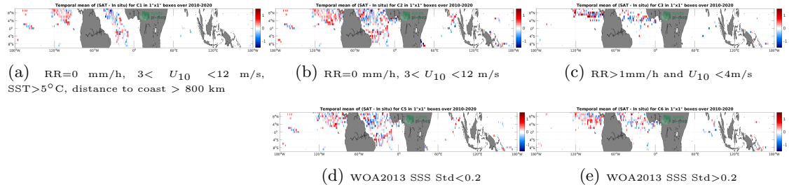
Figure 11: Temporal mean gridded over spatial boxes of size 1^{\circ}\times 1^{\circ} of \Delta\text{SSS} (SMOS SSS L2Q v331 - With FLAG (CMEMS-CATDS-CPDC) - Surface drifters) for 5 different subdatasets corresponding to:RR=0 mm/h, 3 < U_{10} < 12 m/s, SST >5^{\circ}\text{C} , distance to coast > 800 km (a), RR=0 mm/h, 3 < U_{10} < 12 m/s (b), RR >1 mm/h and U_{10} < 4 m/s (c), WOA2013 SSS Std <0.2 (d), WOA2013 SSS Std >0.2 (e).
