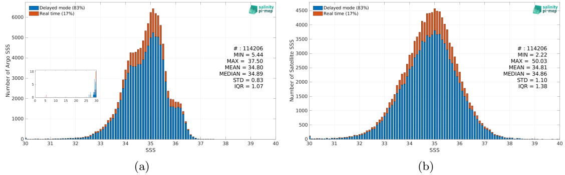
Figure 2: Histograms of SSS from Argo (a) and SMOS SSS L2Q v331 - With FLAG (CMEMS-CATDS-CPDC) (b) considering all match-up pairs per bins of 0.1 over the Equatorial Ocean 10N-10S Pi-MEP region and for the full satellite product period.
