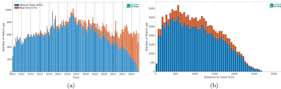
Figure 1: Number of match-ups between Argo and SMOS SSS L2Q v331 - With FLAG (CMEMS-CATDS-CPDC) SSS as a function of time (a) and as function of the distance to coast (b) over the Equatorial Ocean 10N-10S Pi-MEP region and for the full satellite product period.
