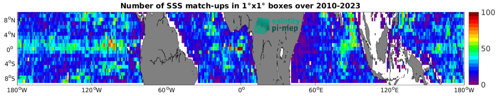
Figure 4: Number of SSS match-ups between Argo SSS and the SMOS SSS L2Q v331 - With FLAG (CMEMS-CATDS-CPDC) SSS product for the Equatorial Ocean 10N-10S Pi-MEP region over 1^\circ \times 1^\circ boxes and for the full satellite product period.
