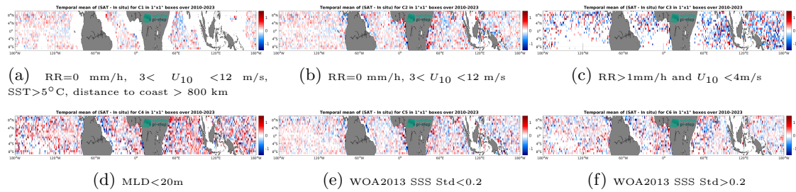
Figure 12: Temporal mean gridded over spatial boxes of size 1^\circ \times 1^\circ of \Delta SSS (SMOS SSS L2Q v331 - With FLAG (CMEMS-CATDS-CPDC) - Argo) for 6 different subdatasets corresponding to:RR=0 mm/h, 3 < U_{10} < 12 m/s, SST >5^\circ C, distance to coast > 800 km (a), RR=0 mm/h, 3 < U_{10} < 12 m/s (b), RR >1 mm/h and U_{10} < 4 m/s (c),MLD <20 m (d),WOA2013 SSS Std <0.2 (e),WOA2013 SSS Std >0.2 (f).
