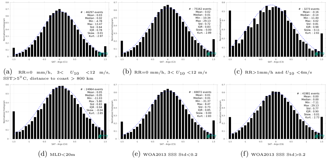
Figure 13: Normalized histogram of \Delta SSS (SMOS SSS L2Q v331 - With FLAG (CMEMS-CATDS-CPDC) - Argo) for 6 different subdatasets corresponding to: RR=0 mm/h, 3 < U_{10} < 12 m/s, SST > 5°C, distance to coast > 800 km (a), RR=0 mm/h, 3 < U_{10} < 12 m/s (b), RR > 1mm/h and U_{10} < 4 m/s (c), MLD < 20m (d), WOA2013 SSS Std < 0.2 (e), WOA2013 SSS Std > 0.2 (f).
