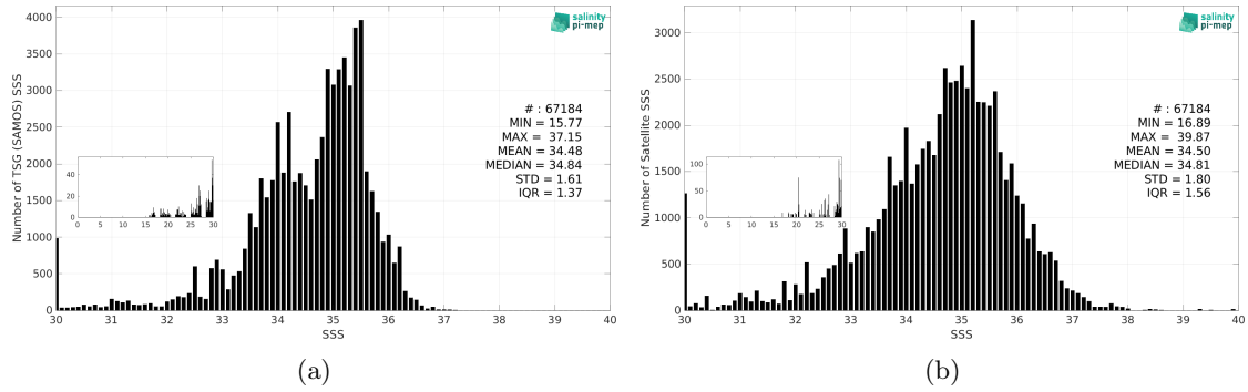
Figure 3: Histograms of SSS from TSG (SAMOS) (a) and SMOS SSS L2Q v331 - No FLAG (CMEMS-CATDS-CPDC) (b) considering all match-up pairs per bins of 0.1 over the Equatorial Ocean 10N-10S Pi-MEP region and for the full satellite product period.
