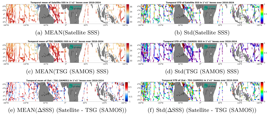
Figure 7: Temporal mean (left) and Std (right) of SSS from SMOS SSS L2Q v331 - No FLAG (CMEMS-CATDS-CPDC) (top), TSG (SAMOS) (middle), and of \Delta SSS (Satellite - TSG (SAMOS)). Only match-up pairs are used to generate these maps.
