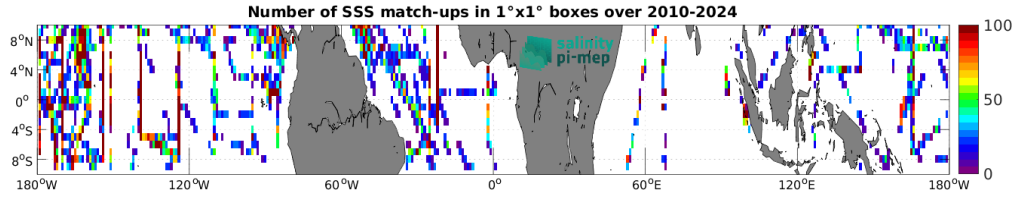
Figure 5: Number of SSS match-ups between TSG (SAMOS) SSS and the SMOS SSS L2Q v331 - No FLAG (CMEMS-CATDS-CPDC) SSS product for the Equatorial Ocean 10N-10S Pi-MEP region over 1^\circ \times 1^\circ boxes and for the full satellite product period.
