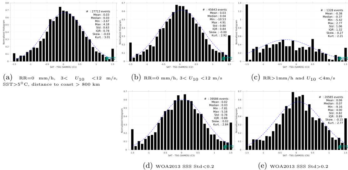
Figure 15: Normalized histogram of \Delta\text{SSS} (SMOS SSS L2Q v331 - No FLAG (CMEMS-CATDS-CPDC) - TSG (SAMOS)) for 5 different subdatasets corresponding to: RR=0 mm/h, 3 < U_{10} < 12 m/s, SST>5°C, distance to coast > 800 km (a), RR=0 mm/h, 3 < U_{10} < 12 m/s (b), RR>1mm/h and U_{10} < 4 m/s (c), WOA2013 SSS Std<0.2 (d), WOA2013 SSS Std>0.2 (e).
