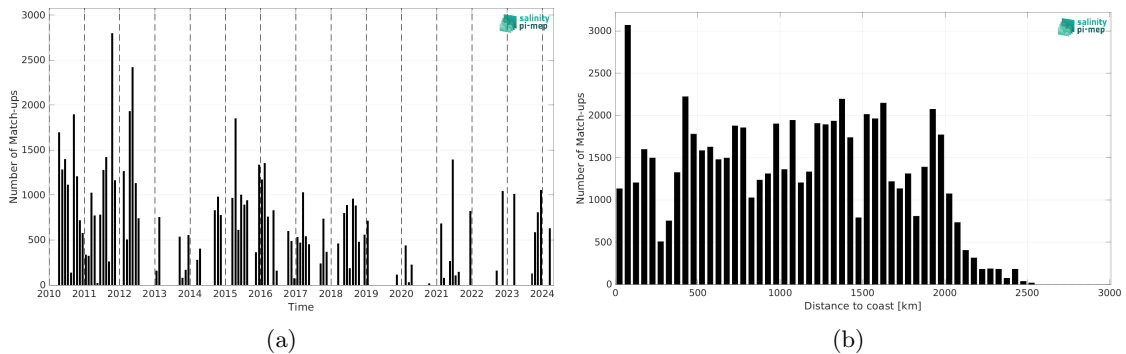
Figure 2: Number of match-ups between TSG (SAMOS) and SMOS SSS L2Q v331 - No FLAG (CMEMS-CATDS-CPDC) SSS as a function of time (a) and as function of the distance to coast (b) over the Equatorial Ocean 10N-10S Pi-MEP region and for the full satellite product period.
