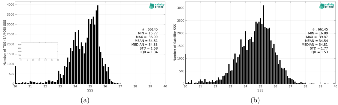
Figure 2: Histograms of SSS from TSG (SAMOS) (a) and SMOS SSS L2Q v331 - No FLAG (CMEMS-CATDS-CPDC) (b) considering all match-up pairs per bins of 0.1 over the Equatorial Ocean 10N-10S Pi-MEP region and for the full satellite product period.
