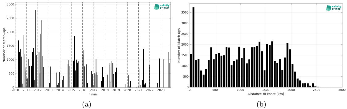
Figure 1: Number of match-ups between TSG (SAMOS) and SMOS SSS L2Q v331 - No FLAG (CMEMS-CATDS-CPDC) SSS as a function of time (a) and as function of the distance to coast (b) over the Equatorial Ocean 10N-10S Pi-MEP region and for the full satellite product period.
