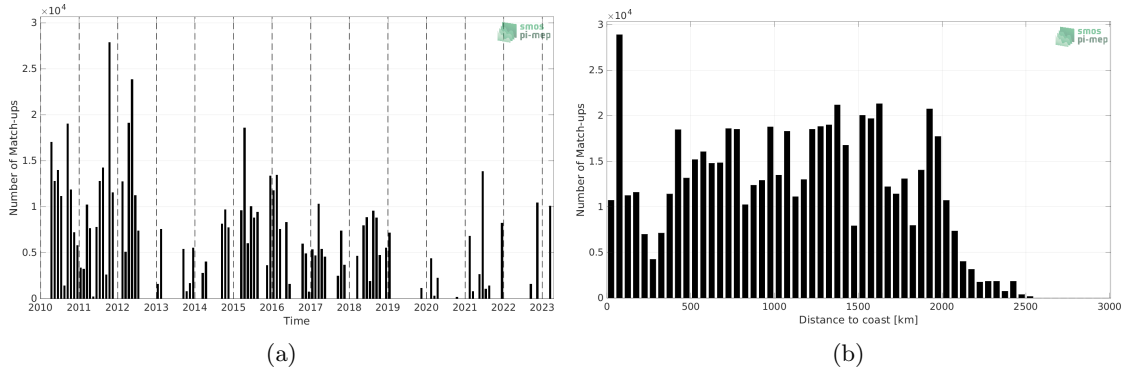
Figure 1: Number of match-ups between TSG (SAMOS) and SMOS SSS L2Q v331 - No FLAG (CMEMS-CATDS-CPDC) SSS as a function of time (a) and as function of the distance to coast (b) over the Equatorial Ocean 10N-10S Pi-MEP region and for the full satellite product period.
