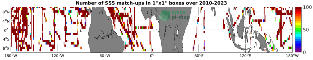
Figure 4: Number of SSS match-ups between TSG (SAMOS) SSS and the SMOS SSS L2Q v331 - No FLAG (CMEMS-CATDS-CPDC) SSS product for the Equatorial Ocean 10N-10S Pi-MEP region over 1^\circ \times 1^\circ boxes and for the full satellite product period.
