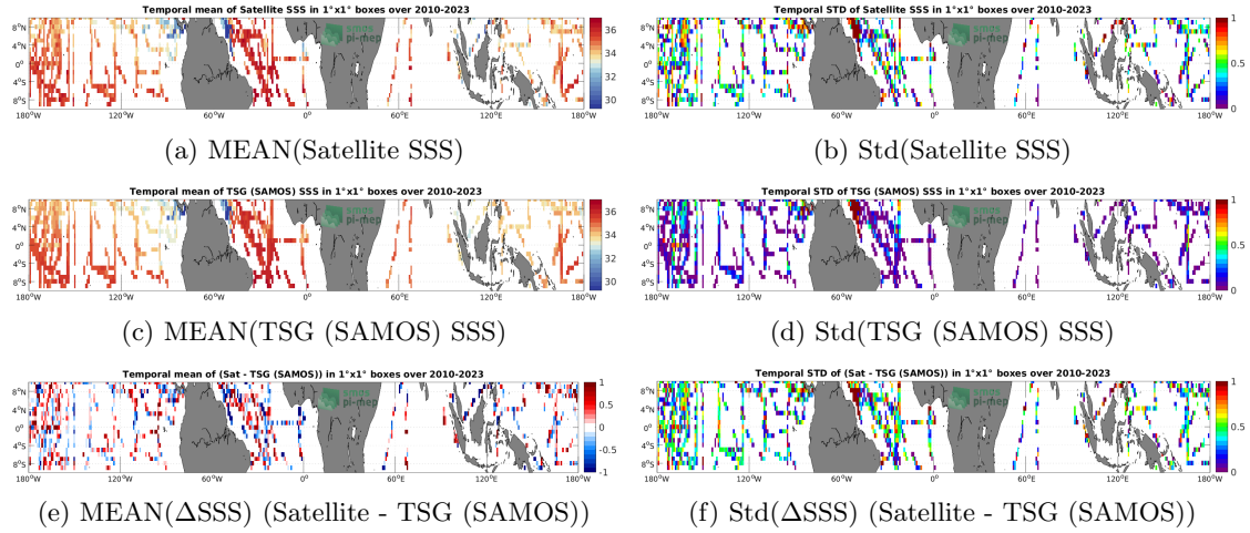
Figure 6: Temporal mean (left) and Std (right) of SSS from SMOS SSS L2Q v331 - No FLAG (CMEMS-CATDS-CPDC) (top), TSG (SAMOS) (middle), and of \Delta SSS (Satellite - TSG (SAMOS)). Only match-up pairs are used to generate these maps.
