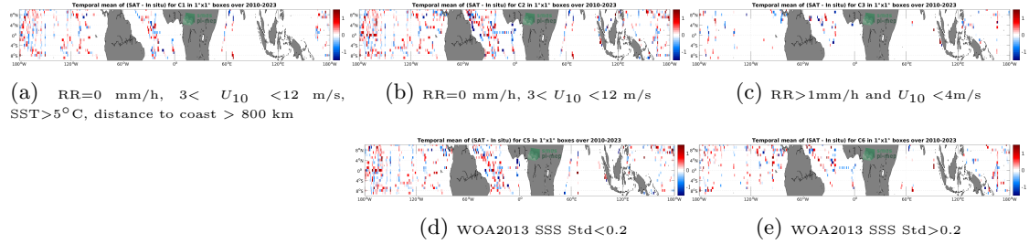
Figure 12: Temporal mean gridded over spatial boxes of size 1^{\circ}\times 1^{\circ} of \Delta\text{SSS} (SMOS SSS L2Q v331 - No FLAG (CMEMS-CATDS-CPDC) - TSG (SAMOS)) for 5 different subdatasets corresponding to:RR=0 mm/h, 3 < U_{10} < 12 m/s, SST >5^{\circ}\text{C} , distance to coast > 800 km (a), RR=0 mm/h, 3 < U_{10} < 12 m/s (b), RR >1 mm/h and U_{10} < 4 m/s (c), WOA2013 SSS Std <0.2 (d), WOA2013 SSS Std >0.2 (e).
