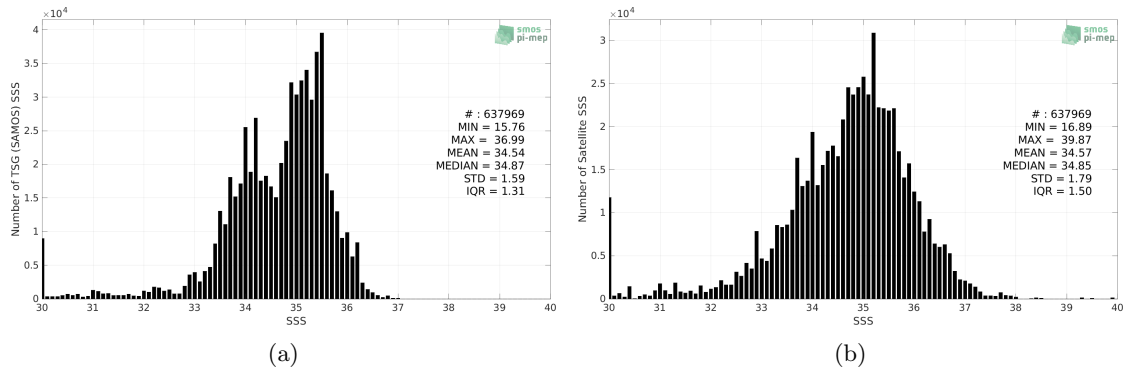
Figure 2: Histograms of SSS from TSG (SAMOS) (a) and SMOS SSS L2Q v331 - No FLAG (CMEMS-CATDS-CPDC) (b) considering all match-up pairs per bins of 0.1 over the Equatorial Ocean 10N-10S Pi-MEP region and for the full satellite product period.
