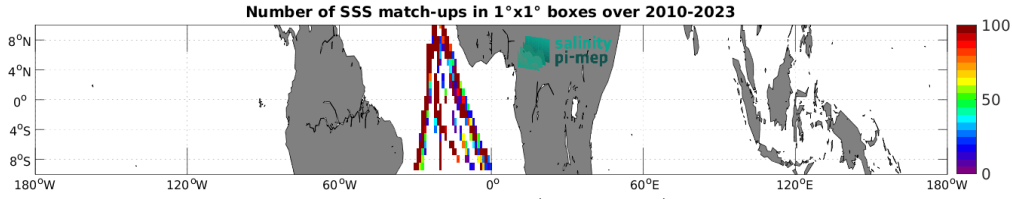
Figure 5: Number of SSS match-ups between TSG (Polarstern) SSS and the SMOS SSS L2Q v331 - No FLAG (CMEMS-CATDS-CPDC) SSS product for the Equatorial Ocean 10N-10S Pi-MEP region over 1^\circ \times 1^\circ boxes and for the full satellite product period.
