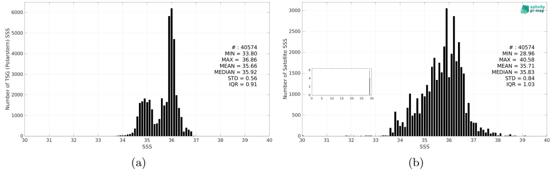
Figure 3: Histograms of SSS from TSG (Polarstern) (a) and SMOS SSS L2Q v331 - No FLAG (CMEMS-CATDS-CPDC) (b) considering all match-up pairs per bins of 0.1 over the Equatorial Ocean 10N-10S Pi-MEP region and for the full satellite product period.
