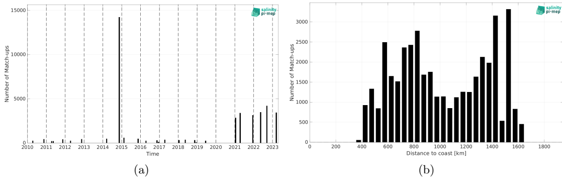
Figure 2: Number of match-ups between TSG (Polarstern) and SMOS SSS L2Q v331 - No FLAG (CMEMS-CATDS-CPDC) SSS as a function of time (a) and as function of the distance to coast (b) over the Equatorial Ocean 10N-10S Pi-MEP region and for the full satellite product period.
