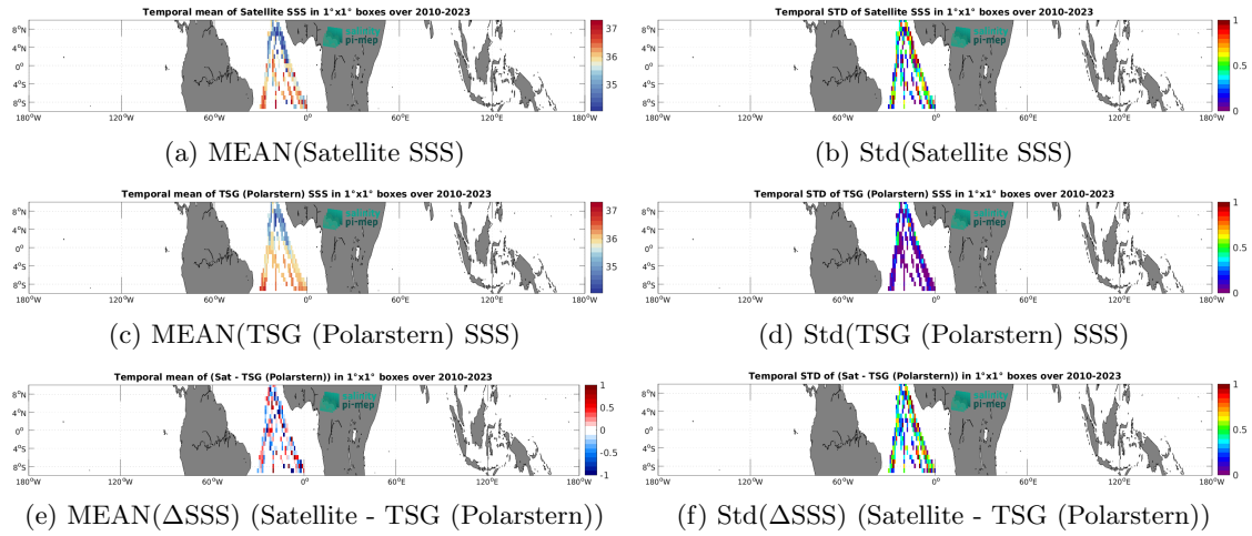
Figure 7: Temporal mean (left) and Std (right) of SSS from SMOS SSS L2Q v331 - No FLAG (CMEMS-CATDS-CPDC) (top), TSG (Polarstern) (middle), and of \Delta SSS (Satellite - TSG (Polarstern)). Only match-up pairs are used to generate these maps.
