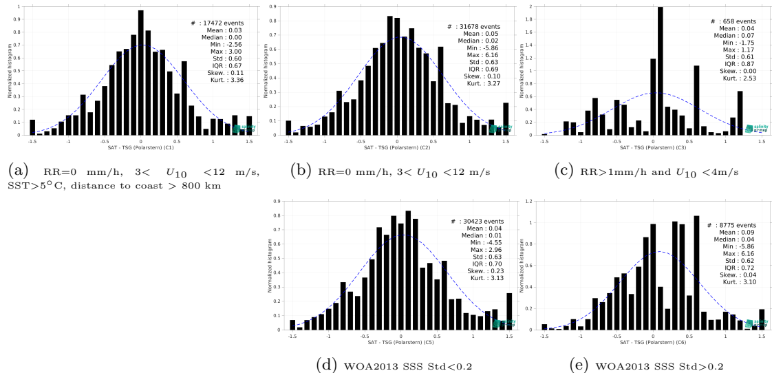
Figure 15: Normalized histogram of \Delta\text{SSS} (SMOS SSS L2Q v331 - No FLAG (CMEMS-CATDS-CPDC) - TSG (Polarstern)) for 5 different subdatasets corresponding to: RR=0 mm/h, 3 < U_{10} < 12 m/s, SST>5°C, distance to coast > 800 km (a), RR=0 mm/h, 3 < U_{10} < 12 m/s (b), RR>1mm/h and U_{10} < 4 m/s (c), WOA2013 SSS Std<0.2 (d), WOA2013 SSS Std>0.2 (e).
